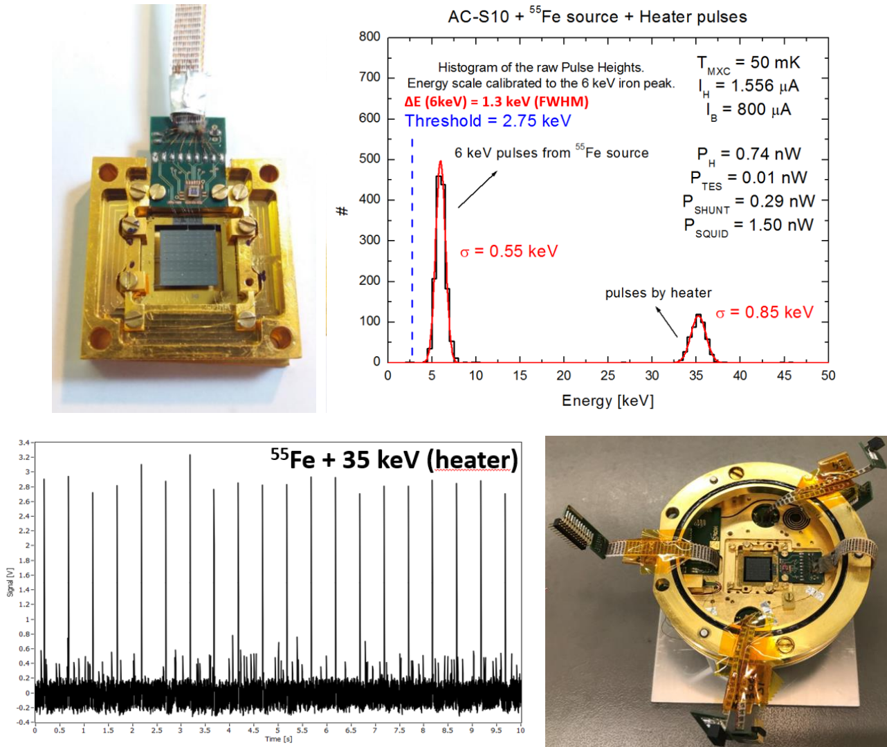
Fig. 4 - Top left DM: CryoAC in INAF holder. Top right: Energy spectrum from ^{55}\text{Fe} , and 35 keV pulses injected by the heater. Bottom left Raw data stream. Bottom right fit-checking in the 40 PxIB flange at SRON (credits SRON).
