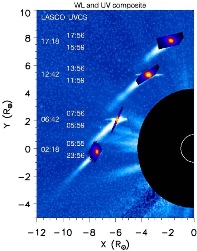
Figure 7. Composite comet image of visible light from LASCO C3 and reconstructed H I \text{Ly}\alpha intensity from UVCS spectra. The labels report the observation times of LASCO C3 and the time interval of the UVCS observation.
