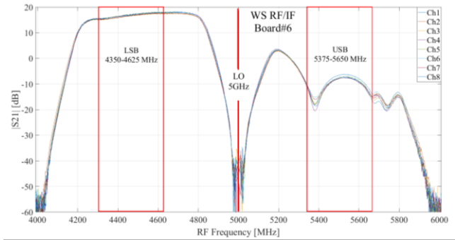
Fig. 9. VNA measured transmissions of the eight channels of the WS RF/IF boards by selecting filter BPF-A and LO frequency 5 GHz.
