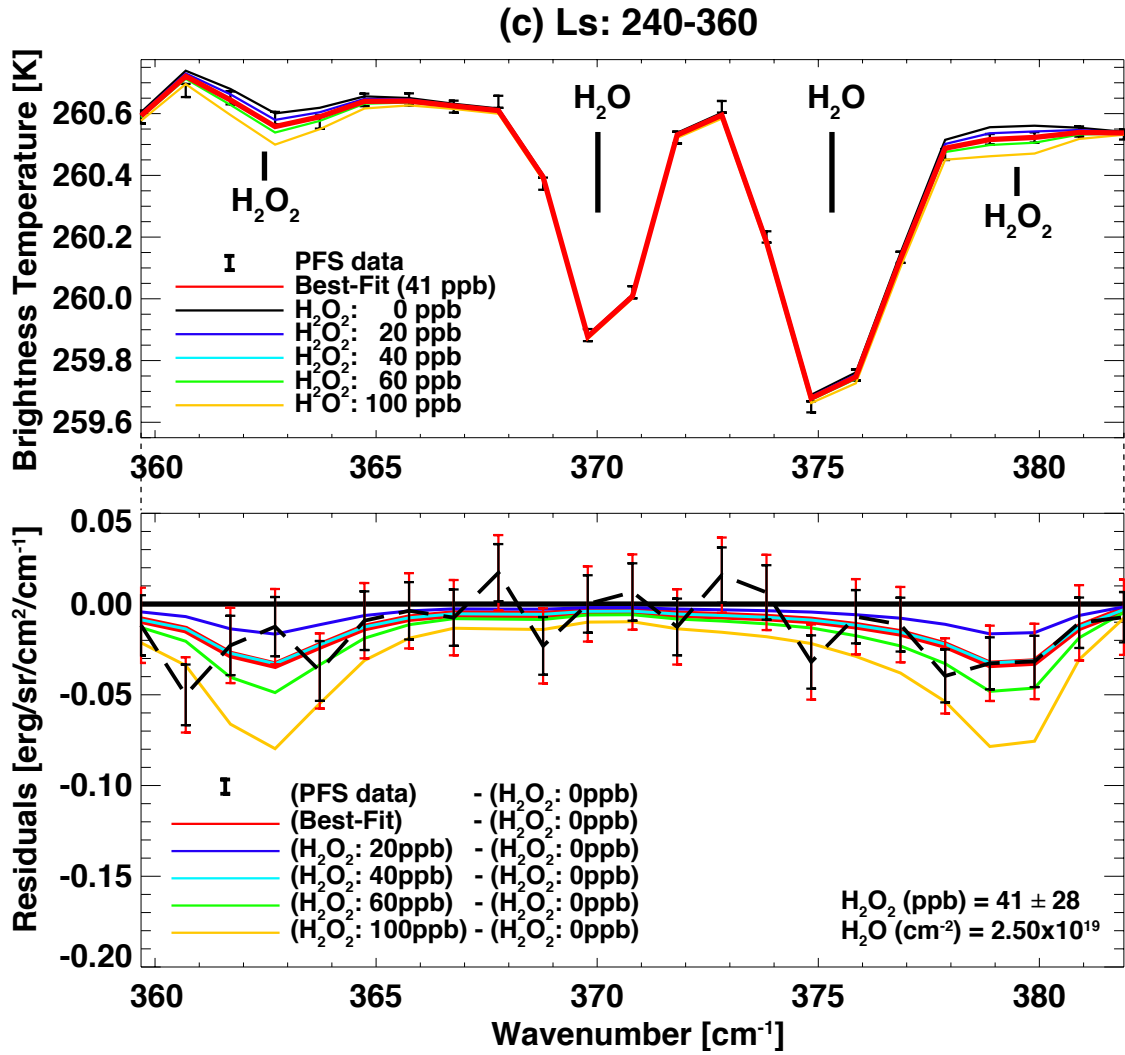
Figure 3. The PFS averaged spectra over (a) L_s = 0-120^\circ , (b) L_s = 120-240^\circ , and (c) L_s = 240-360^\circ in the spectral range between 359 and 382 \text{cm}^{-1} . (Top) Comparison between the synthetic spectra and the averaged PFS spectra. The red curves show the best-fit synthetic spectra. The other color curves represent synthetic spectra with various mixing ratios of \text{H}_2\text{O}_2 (blue: 20 ppb, light blue: 40 ppb, green: 60 ppb, orange: 100 ppb). The black vertical bars show instrumental noise calculated by the noise equivalent radiance divided by the square root of the number of measurements. (Bottom) Residual spectra, where special synthetic spectra with all contributions except \text{H}_2\text{O}_2 have been subtracted from the measured and synthetic (including \text{H}_2\text{O}_2 contribution) spectra. The retrieved \text{H}_2\text{O}_2 values are 16 \pm 19 ppb at L_s =
