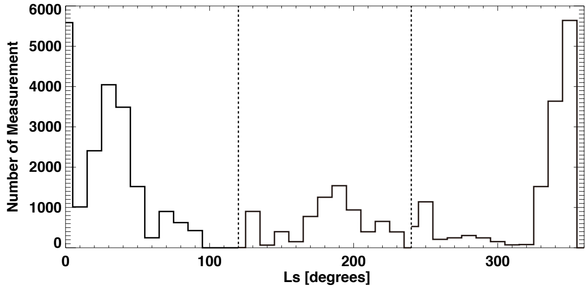
Figure 2. The distributions of solar longitude L_s in the three datasets that were used. The histogram shows the numbers of measurements as a function of the solar longitude. The interval of the histogram is 10^\circ .
