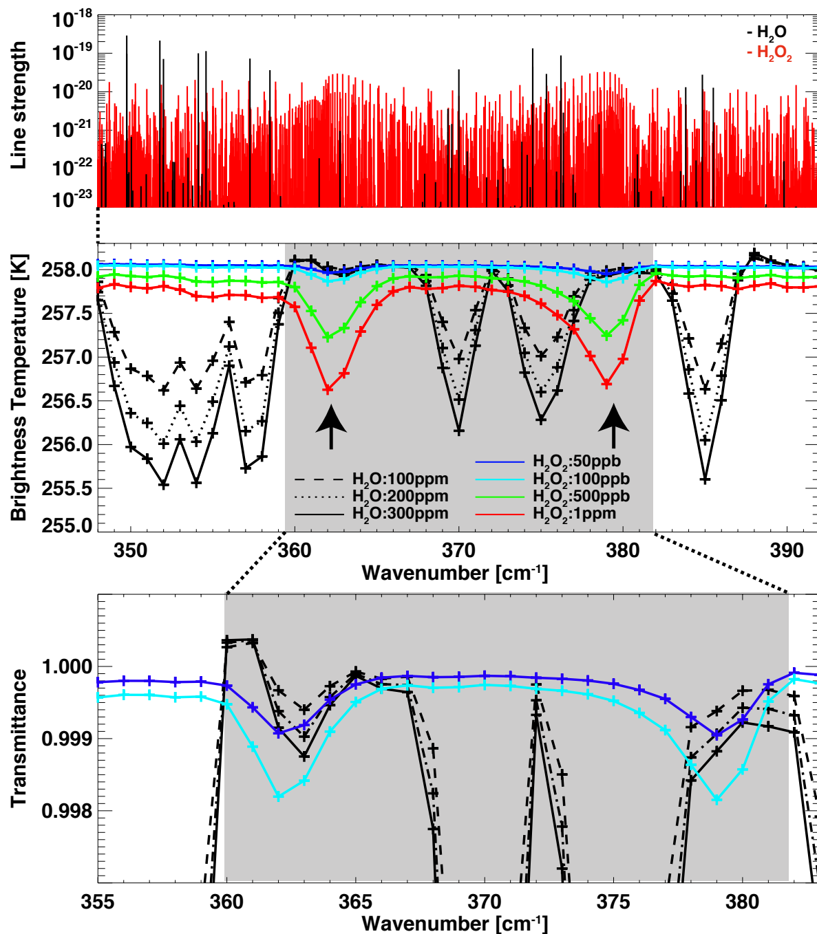
Figure 1. (Top) Line strength of H 2 O and H 2 O 2 in the spectral range between 350 and 390 cm -1 obtained from HITRAN08. (Middle) Synthetic spectra in the spectral range between 350 and 390 cm -1 with the spectral resolution of the apodized PFS spectrum. The black curves show the spectra with various mixing ratios of H 2 O (dash: 100 ppm, dot: 200 ppm, solid: 300 ppm). The color curves show the spectra with various mixing ratios of H 2 O 2 (blue: 50 ppb,
