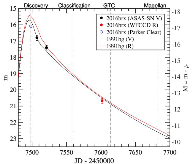
Figure A2. The available V- and R-band photometry of SN 2016brx (black and red solid dots) are matched with those of the SN 1991bg (black and red lines) by applying the same magnitude shift in both bands and a shift in time. We also show the magnitude subtracted by the distance modulus \mu = 33.2 on the right y-axis. We also show the clear-filter discovery magnitude of SN 2016brx taken by Stuart Parker (blue open circle). The time of discovery, spectroscopic classification, GTC and Magellan spectra are marked with black dashed lines.
