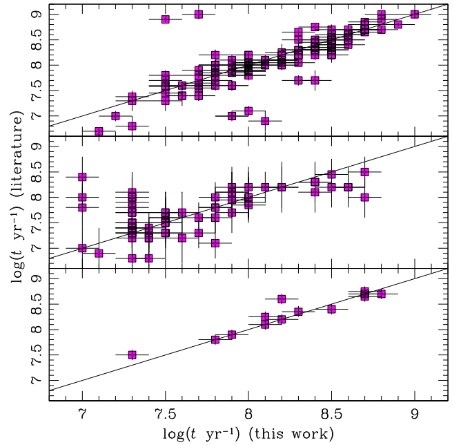
Figure 4. Comparison of the cluster age estimates derived here with those from the literature: PU00 (top panel), G10 (middle panel) and Washington photometry (Piatti 2012, 2014b; Choudhury, Subramanian & Piatti 2015, bottom panel). Error bars and the locus of equality are also shown.
