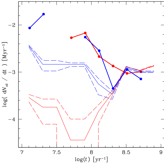
Figure 10. CFs for subregions D1 (thick red line) and D2 (thick blue line) in tile LMC 6_6. Thin and dashed lines represent, respectively, the mean CFs and their 1\sigma dispersions recovered from the corresponding SFRs obtained by Rubele et al. (2012).
