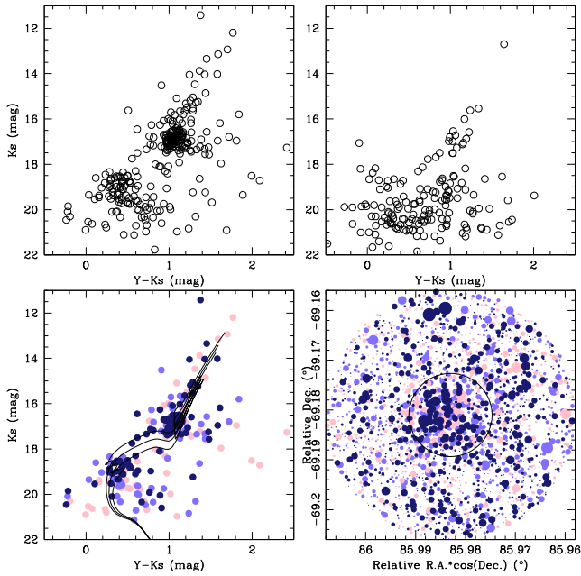
Figure 2. CMDs for stars in the field of NGC 2108: the observed CMD composed of the stars distributed within the cluster radius (top-left panel); a field CMD for an annulus – outer and inner radii equal to 3.163 and 3.0 times the cluster radius – centred on the cluster (top-right panel); the cleaned cluster CMD (bottom-left). Colour-scaled symbols represent stars that statistically belong to the field ( P \leq 25 per cent, pink), stars that might belong to either the field or the cluster ( P = 50 per cent, light blue), and stars that predominantly populate the cluster region ( P \geq 75 per cent, dark blue). Three isochrones from Bressan et al. (2012) for \log(t \text{ yr}^{-1}) = 8.8, 8.9 , and 9.0 and Z = 0.006 are also superimposed. The lack of fainter main-sequence stars results in less satisfactory matching at fainter magnitudes. The schematic diagram centred on the cluster for a circle of radius three times the cluster radius is shown in the bottom-right panel. The black circle represents the adopted cluster radius. Symbols are as in the bottom-left panel, with sizes proportional to the stellar brightnesses. North is up; east is to the left.
