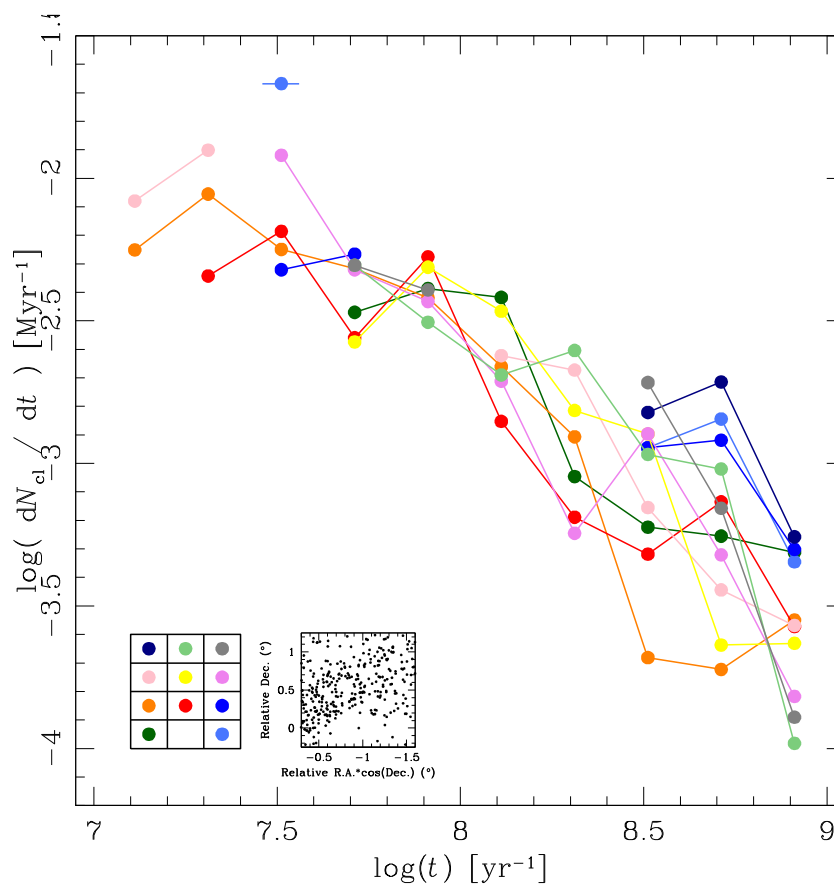
Figure 6. CFs for subregions in tile LMC 6_4. The bottom-right hand panel shows the spatial distribution of the Bica et al. (2008) catalogue of star clusters, while the left-hand panel schematically represents the subregions and indicates the colour used in drawing the respective CFs. North is up and east is to the left. Note that computed values (filled circles) for each CF are connected by a solid line. Some CFs do not have points for certain age intervals because of the lack of clusters within them, which resulted in truncated CFs. In such cases, we drew isolated points with a short line to represent that they belong to a truncated CF. One subregion does not contain any cluster in our sample.
