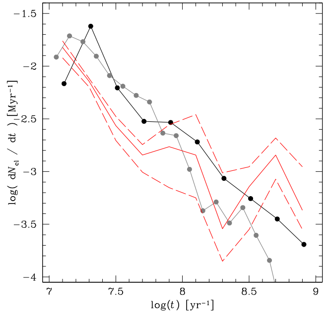
Figure 9. As Fig. 8, but for tile LMC 6_6 and HZ09's 30 Doradus region.
