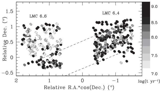
Figure 5. Spatial distribution of the cluster ages, with darker shading representing older ages, centred at RA = 05^{\text{h}}23^{\text{m}}34^{\text{s}} , Dec. = -69^{\circ}45'22'' (J2000). North is up; east is to the left. The grey-scale is in units of \log(t \text{ yr}^{-1}) . The locations of 30 Doradus and the LMC bar are indicated with a dashed circle and two parallel lines (Subramaniam & Subramaniam 2009), respectively.
