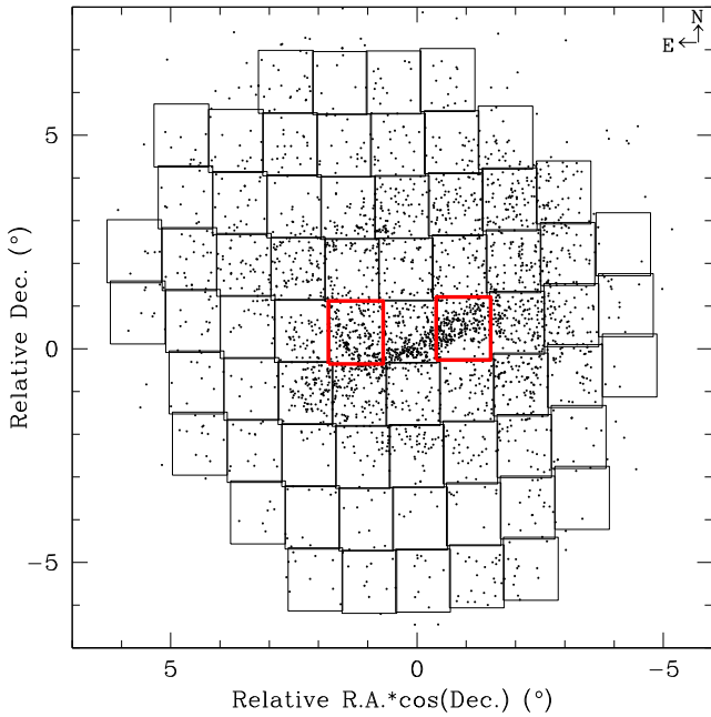
Figure 1. Spatial distribution of the Bica et al. (2008) catalogue of star clusters in the LMC centred at RA = 05 h 23 m 34 s , Dec. = −69°45′22″ (J2000), projected on to the sky. The objects studied in this paper are located in tiles highlighted as red rectangles: LMC 6_4 (right) and LMC 6_6 (left). The remaining VMC tiles across the LMC are shown as black rectangles.
