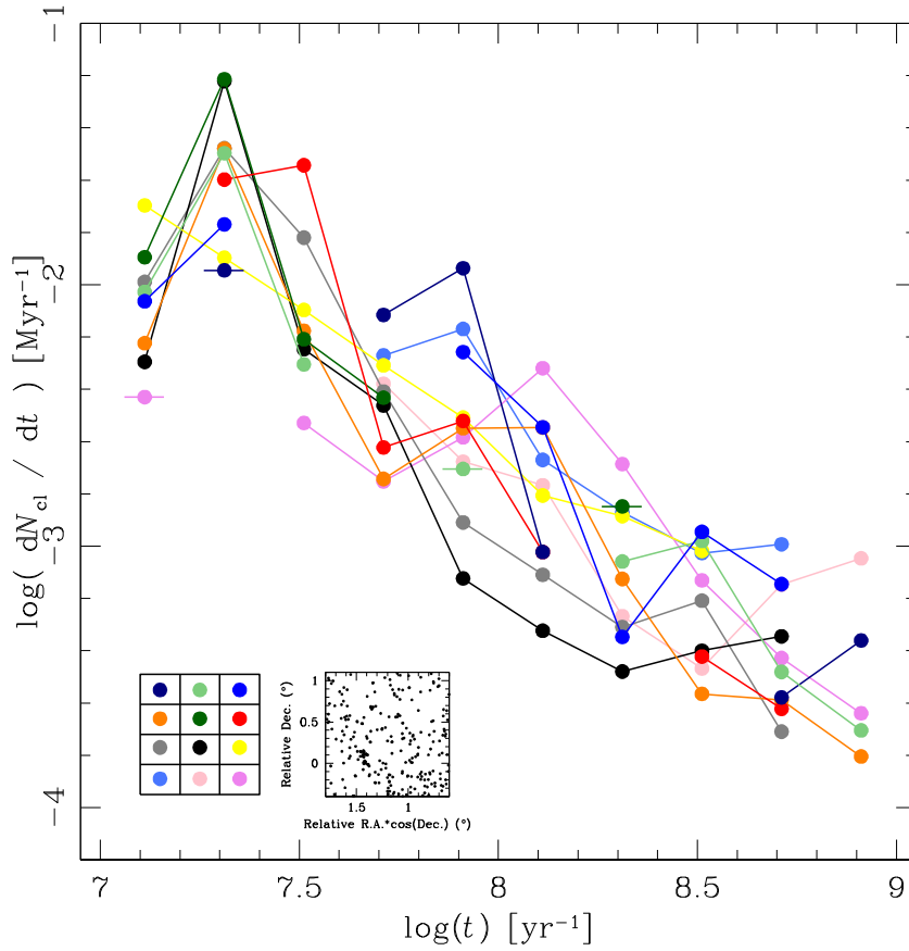
Figure 7. As Fig. 6, but for tile LMC 6_6.
