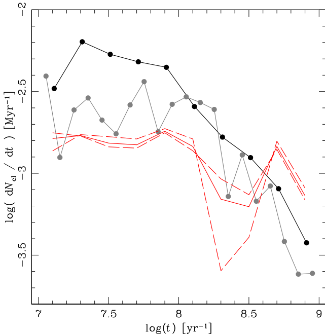
Figure 8. Composite CF for tile LMC 6_4 (black) compared with those obtained by P14 for clusters within HZ09's bar region (grey) and by HZ09 for the respective mean SFR and its 1\sigma uncertainty (solid and dashed red lines, respectively).
