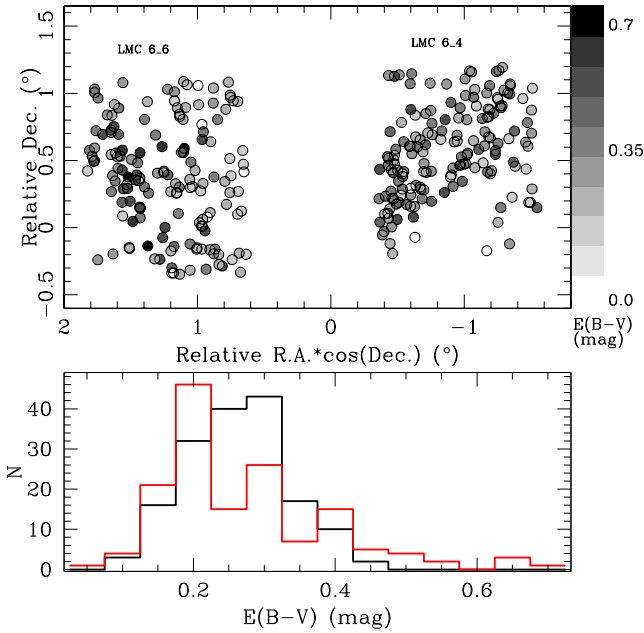
Figure 3. Reddening histograms for tiles LMC_6_4 (black) and LMC_6_6 (red; bottom panel) and the spatial distribution of the clusters’ reddening, with darker shading representing higher reddening values (top panel). The grey-scale is in units of E(B - V) (mag).
