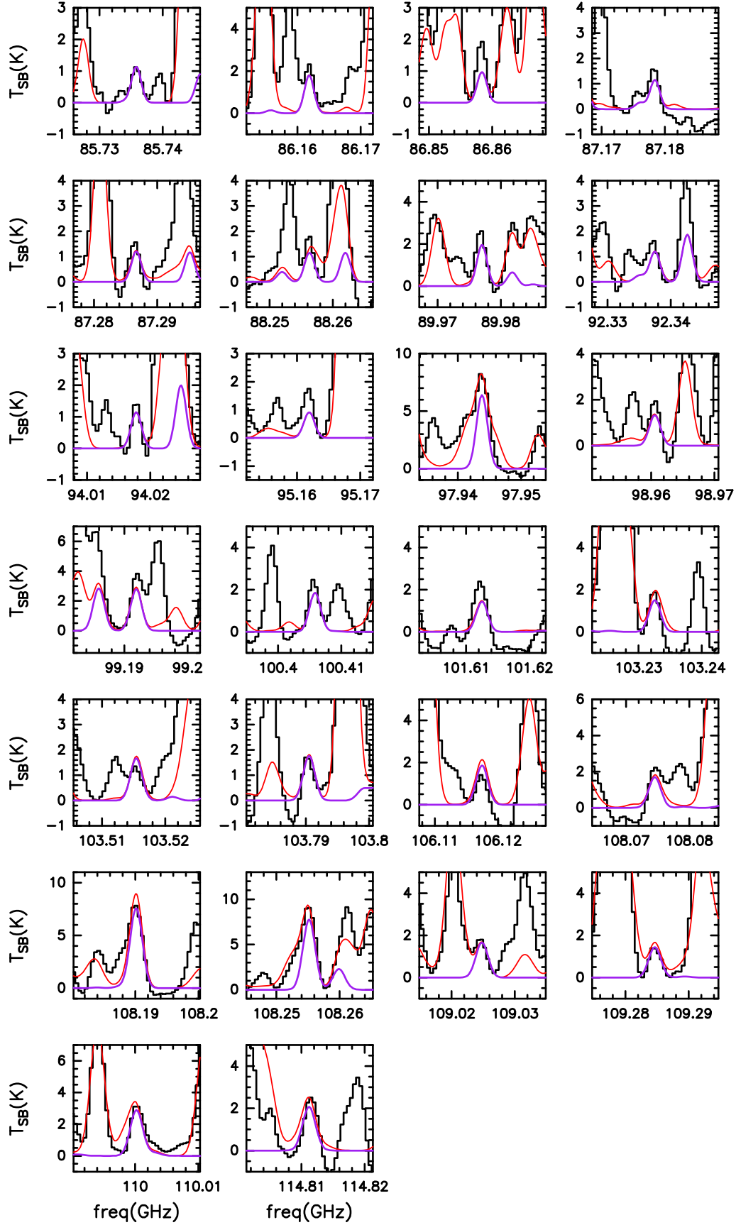
Fig. 8. Transitions listed in Table C.1 and used to fit the v=0 , and v_t=1, 2 states of acetamide ( \text{CH}_3\text{C(O)NH}_2 ). The purple curve represents the best LTE fit obtained with MADCUBA (Table 1). The red curve shows the simulated spectrum taking into account all the species identified so far in the region.
