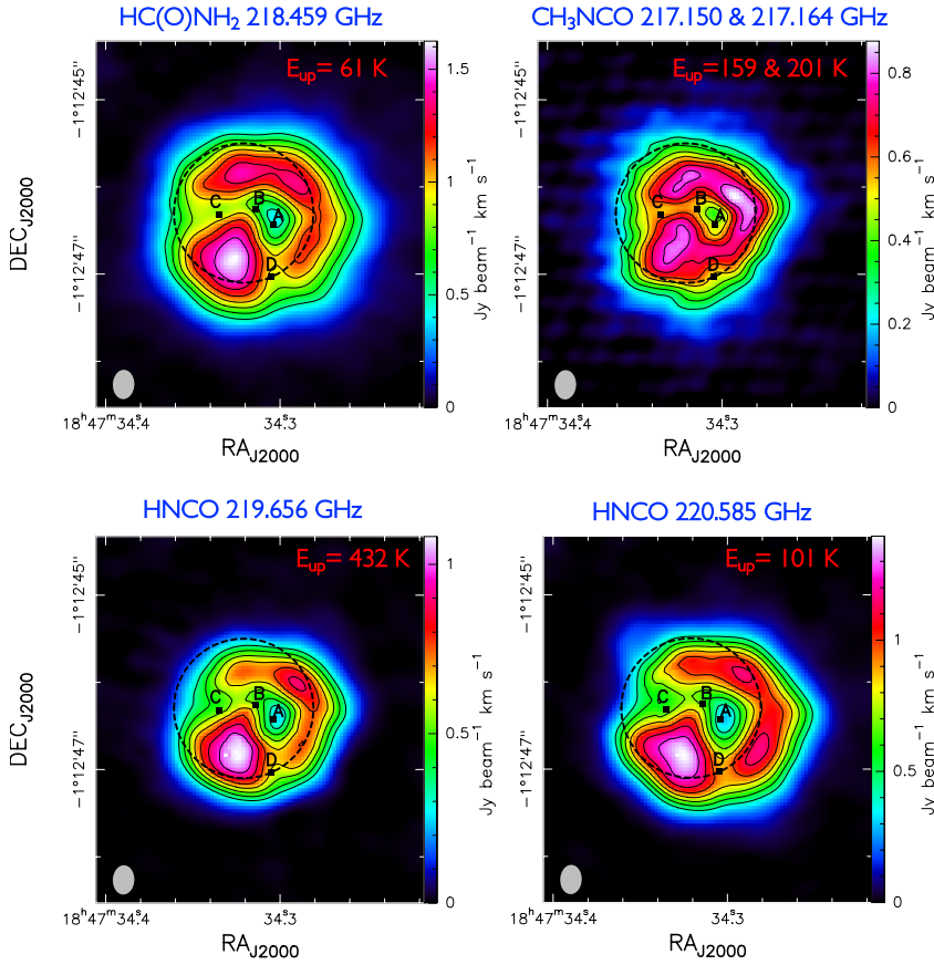
Fig. 13. ALMA 0.2 resolution integrated emission maps at 1.4 mm of \text{HC(O)NH}_2 ( 10_{1,9-9_{1,8}} ) (top-left panel), \text{CH}_3\text{NCO} ( 25_{2,23,0-24_{2,22,0}} and 25_{-3,-1-24_{-3,-1}} ) (top-right panel), \text{HNCO} ( 10_{3,8-9_{3,7}} and 10_{3,7-9_{3,6}} ) (bottom-left panel), and \text{HNCO} ( 10_{1,9-9_{1,8}} ) (bottom-right panel) in a velocity range between 93 and 100 \text{km s}^{-1} for each transition. The contour levels are 0.3, 0.4, 0.5, 0.6, 0.7, 0.8, and 0.9 the maximum value of the maps. The maximum values of the maps are 1.625 \text{Jy beam}^{-1} \text{km s}^{-1} for \text{HC(O)NH}_2 , 0.877 \text{Jy beam}^{-1} \text{km s}^{-1} for \text{CH}_3\text{NCO} , 1.082 \text{Jy beam}^{-1} \text{km s}^{-1} for \text{HNCO} at 219.656 GHz, and 1.396 \text{Jy beam}^{-1} \text{km s}^{-1} for \text{HNCO} at 220.585 GHz. The black dashed circle indicates in all the panels the area in which the spectrum analysed in this work was extracted, which matches the GUAPOS beam of 1.2 centered at the 3mm continuum peak. The frequency and E_{\text{up}} energies of the transitions are shown in blue above each panel, and in red in the top-right corner of each panel, respectively. The synthesised beam is represented by the grey ellipse in the lower left corner. The black squares indicates the position of the continuum sources A, B, C, and D resolved with 7 mm VLA observations by Beltrán et al. (2021).
