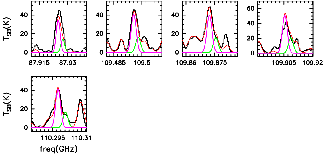
Fig. 2. Transitions listed in Table C.1 and used to fit the v=0 state of isocyanic acid (HNCO) and its ^{13}\text{C} -isotopologue ( \text{HN}^{13}\text{CO} ). The magenta and green curves represent the best LTE fits obtained with MADCUBA for HNCO and \text{HN}^{13}\text{CO} , respectively (Table 1). The red curve shows the simulated spectrum taking into account all the species identified so far in the region.
