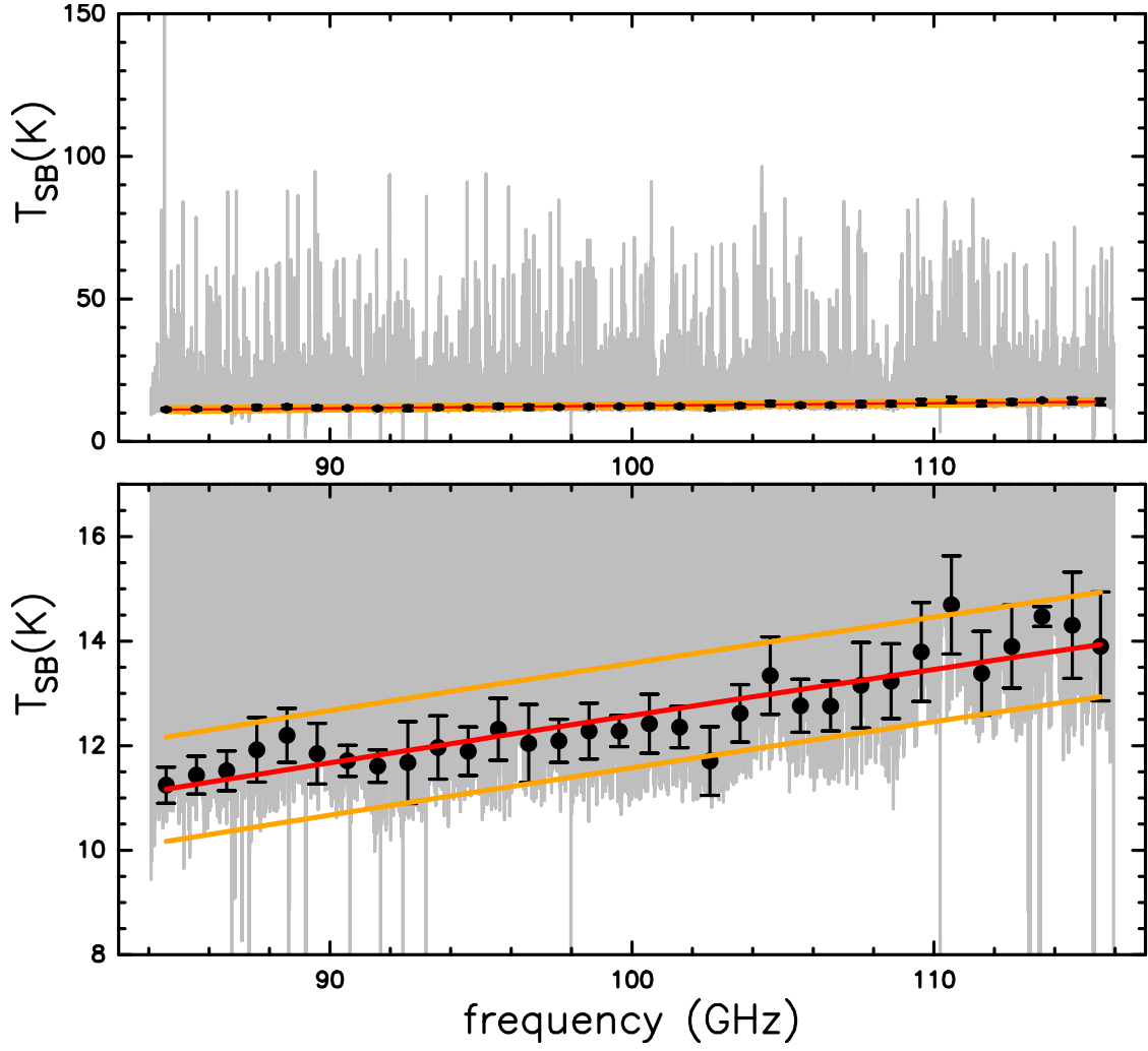
Fig. A.1. Top panel: Continuum level derived with STATCONT overimposed to the GUAPOS spectrum. Bottom panel: y-axis zoom of the top panel. The solid line represents the result from the linear regression fit, as explained in Appendix A, and the orange lines represent the error of \pm 1 K on the fit.
