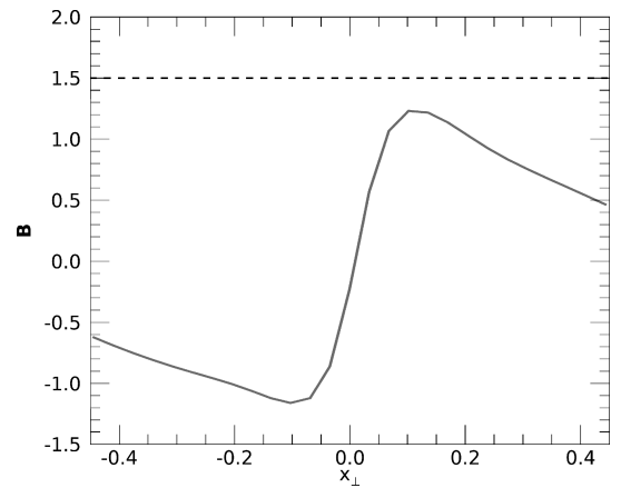
Figure 8. The solid curve represents the variation of the reconnecting field in the direction normal to the current sheet at a selected position (the central point has coordinates x = 2 , y = 1 , z = 15 ) at t = 40 , around the maximum of the integral of J^2 . The dashed line indicates the value of the average guide field in the represented space interval. x_\perp indicates the coordinate normal to the current sheet.
