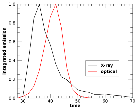
Figure 10. Plot of the total emission in the X-ray (black) and optical (red) bands as a function of time. Each curve is normalized to its maximum value.
