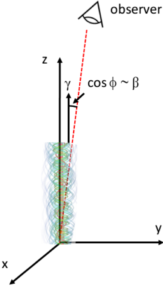
Figure 1. Sketch of the geometry of the model. The jet moves along the z direction with velocity \beta , corresponding to a Lorentz factor \gamma = 10 . The observer lies in the y - z plane and his line of sight forms an angle \phi with the jet direction, such that \cos \phi \sim \beta .
