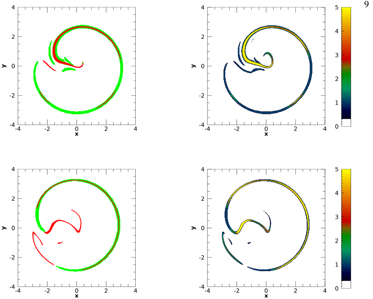
Figure 9. The panels on the left show the positions of the particles in a transverse ( x - y ) section of the jet at z = 10 , in green we show particles that have an age less than r_j/c and in red the particles that have an age between 3r_j/c and 10r_j/c . The panels on the right show instead the density of particles in the same section of the jet. The panels on top refer to t = 40 , around the maximum of the integral of J^2 , while the panels at the bottom refer to t = 46 , in the decreasing phase of the current.
