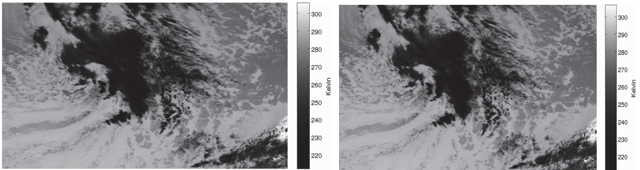
Figure 3. Stereo image pair. MSG-2 and MSG-3 scene 06/02/2015 h:15:12 UTC, Brightness Temperatures in 10.8 \mu\text{m} band. The coldest then the highest clouds, are represented by the darkest colour. Brightest areas represent ocean and land.
