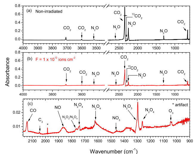
Figure 1. Infrared spectra showing radiolysis effects on N 2 O:CO 2 ice: (a) spectrum of the non- irradiated ice mixture from 4000 to 600 cm -1 ; (b) spectrum after 1.0 × 10 12 ions cm -2 ; and (c) zoom of the previous spectrum, in the 2170 to 900 cm -1 region. The N 2 O 3 band peaked at 1305 cm -1 appears as a shoulder band after de-convolution of the N 2 O fundamental band (1296 cm -1 ).
