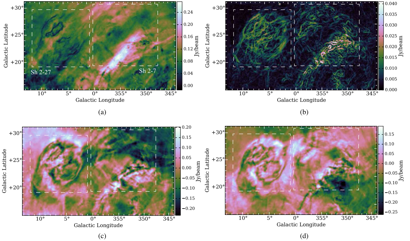
Figure 10. A subregion of the S-PASS survey including the H II regions Sh 2-7 and Sh 2-27. (a) shows the polarized intensity, (b) shows the |\nabla \mathbf{P}| map at its original resolution, and the E - and B -mode maps associated with the same region are shown in (c) and (d).
