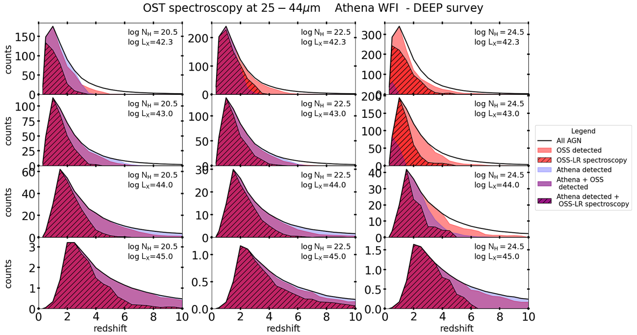
Figure 6. Number of AGN expected per \text{deg}^2 and per \Delta z = 1 for a OSS DEEP survey. The lines and areas are coded as in Figure 5, but with the red areas referring to the band 1 of the OST OSS instrument.
