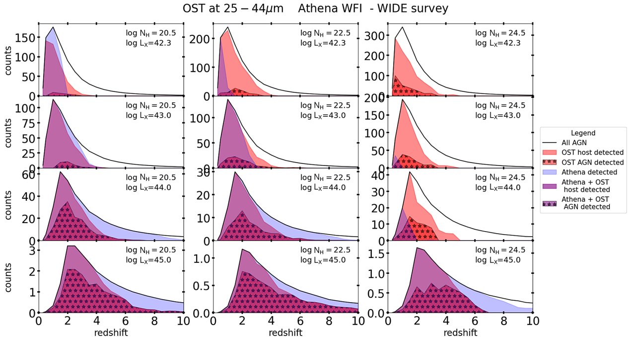
Figure 4. Number of AGN expected per \text{deg}^2 and per \Delta z = 1 for a OST OSS WIDE survey. The lines and areas are coded as in Figure 3.
