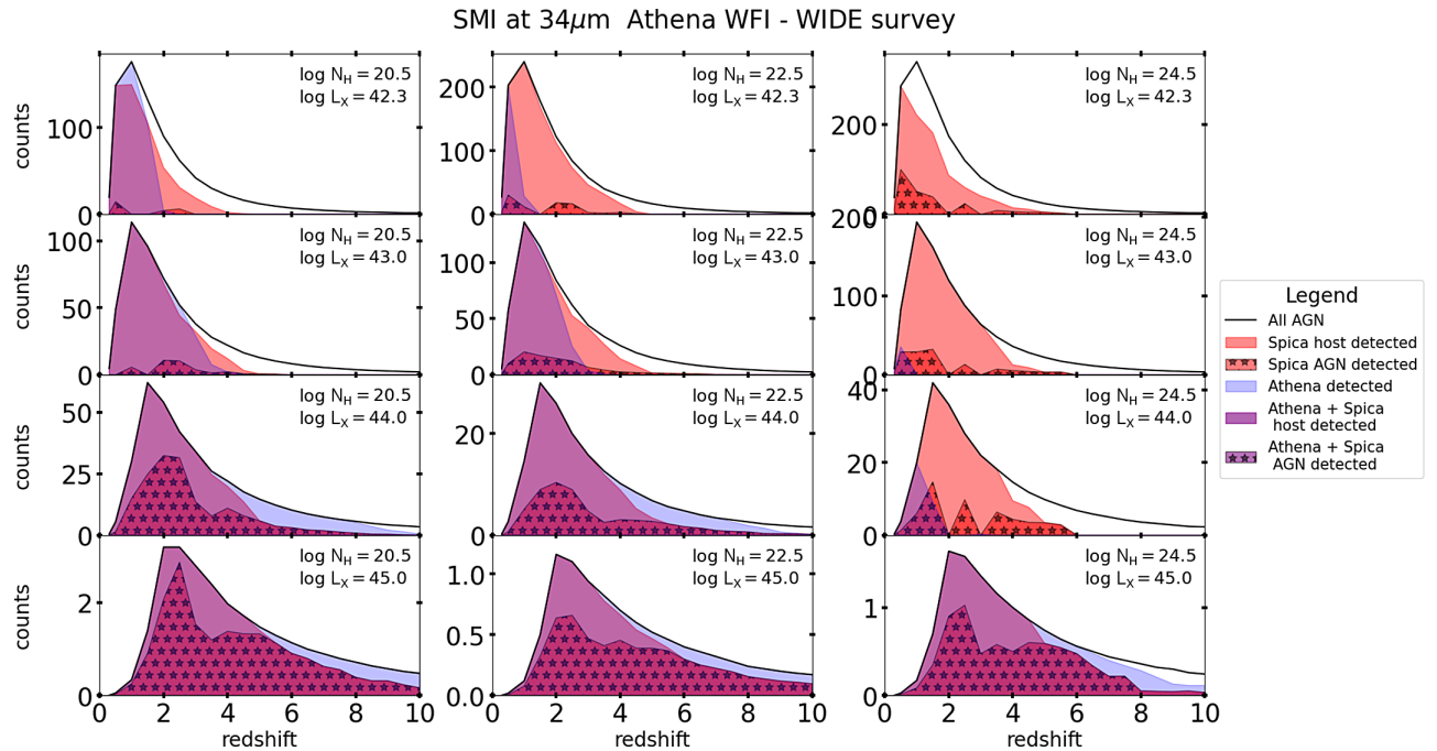
Figure 2. Number of AGN expected per \text{deg}^2 and per \Delta z = 1 for a SPICA -like WIDE survey. The lines and areas are coded as in Figure 1.
