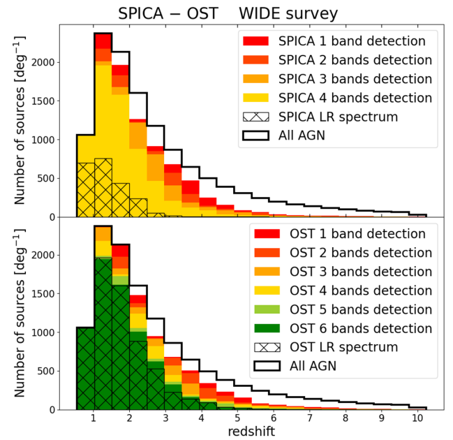
Figure 8. Distribution of the number of AGN expected per \text{deg}^2 for a SPICA-like (top panel) and for the OST OSS (bottom panel) from a WIDE survey. The lines and areas are coded as in Figure 7.
