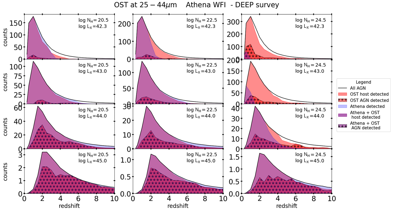
Figure 3. Number of AGN expected per \text{deg}^2 and per \Delta z = 1 for a OST OSS DEEP survey. The black lines are the total number of expected AGN, the red areas represent those which can be detected in the band 1 by OST OSS, the blue areas those which can be detected in the X-rays with the Athena WFI, and the purple areas are the AGN that will be detected both by OSS and Athena. The red uniform area represents the sources detected by OSS in which the main component is due to the host galaxy emission, while for those represented with the starry red area the AGN is the main contributor to the detected emission. The columns refer to AGN with different amount of obscuration ( 20 \leq \log(N_H/\text{cm}^{-2}) \leq 21 ; 22 < \log(N_H/\text{cm}^{-2}) \leq 23 ; 24.18 < \log(N_H/\text{cm}^{-2}) \leq 25 , from left to right), the rows to different AGN luminosity ( 42.0 \leq \log(L_X/\text{erg s}^{-1}) < 42.3 , 42.9 \leq \log(L_X/\text{erg s}^{-1}) < 43.2 , 43.9 \leq \log(L_X/\text{erg s}^{-1}) < 44.2 , 44.9 \leq \log(L_X/\text{erg s}^{-1}) < 45.2 , from top to bottom). For 40 times we extracted 20 SEDs for each bin, we measured the flux in each OST band and compared them with the 5\sigma sensitivities to compute the number of detectable sources. The median of these 40 values are the numbers used in this figure, while the 84–16th percentiles are used as uncertainties (not reported in the figure).
