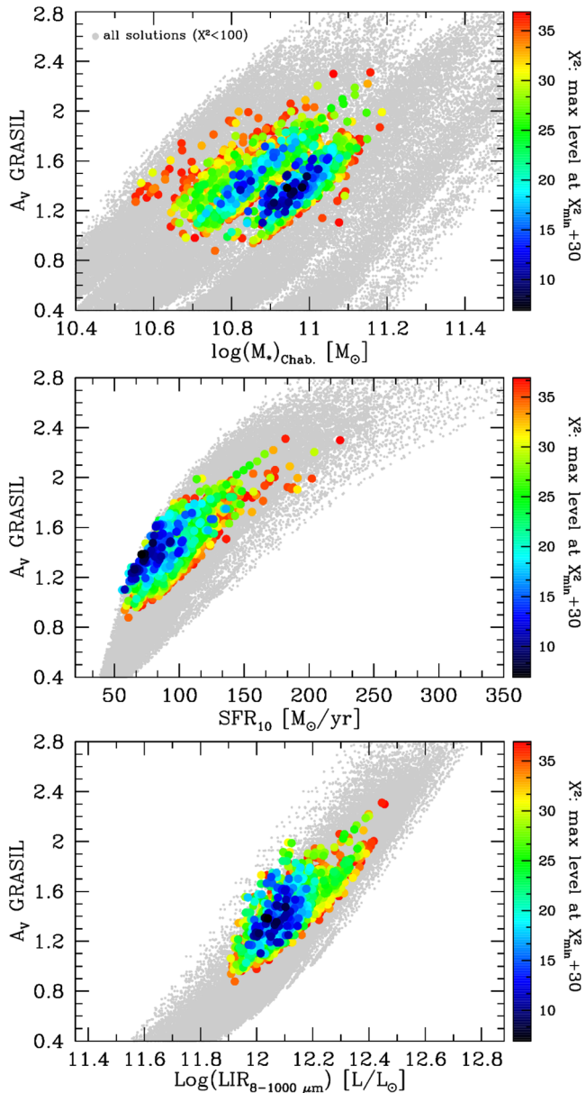
Figure 8. \chi^2 values for spectral models of a typical z \sim 2 ULIRG colour coded ( \chi^2 increasing from dark to light colours) as a function of the average extinction and the stellar mass (top), SFR (centre) and TIR luminosity (bottom). We show here all the solutions with \chi^2 \leq 100 (grey dots) in order to give an idea of the wide range of parameters (and solutions) explored, at fixed geometry, and those with \chi^2 within \chi^2_{\min} + 30 (coloured points). In addition to the variation of the input GRASIL parameters fully discussed in BLF13, we consider here also the variation of the two parameters characterizing the SFH, namely \nu_{\text{Sch}} and \tau_{\text{inf}} . As evident from the figure not much degeneracy is seen among the model parameters. The typical uncertainty on our best-fitting M_* , A_V , \text{SFR}_{10} and L_{\text{IR}} are, respectively, 0.2 dex, 0.3 mag, 0.2 dex and 0.13 dex thus well within the typical uncertainties for this kind of analysis.
