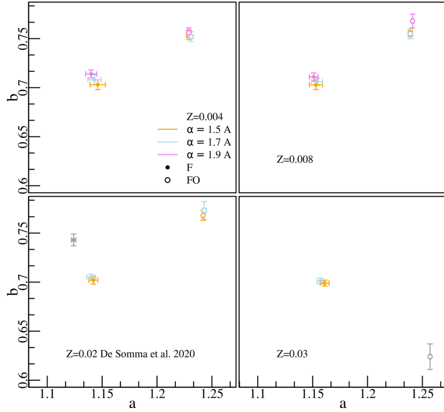
Figure 2. Intercept ( a ) and the slope ( b ) of the fitted canonical F and FO-mode PR relations for Z = 0.004 and Y = 0.25 , Z = 0.008 and Y = 0.25 , Z = 0.02 and Y = 0.28 (taken from De Somma et al. 2020b), and Z = 0.03 and Y = 0.28 as a function of the mixing length parameter (see the main text and labels for more details).
