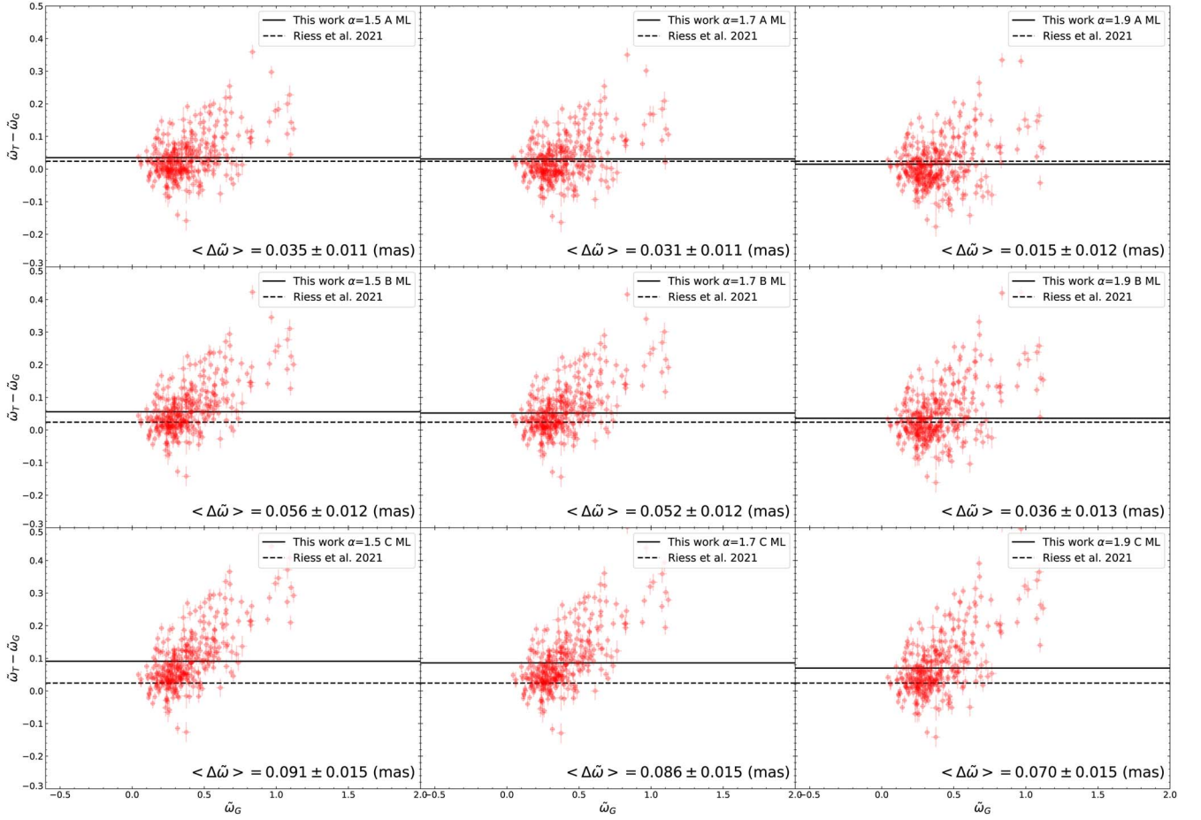
Figure 13. The same as Figure 12 but with the theoretical parallaxes obtained by applying the PW relation for Z = 0.02 .
