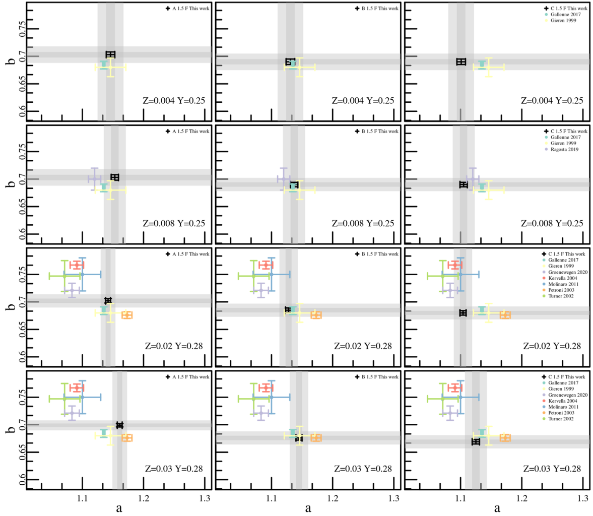
Figure 4. Intercept ( a ) and the slope ( b ) of the fitted theoretical PR relations for the F-mode pulsators and \alpha_{ml} = 1.5 are compared to independent results available in the literature. The different panels show the results for different metallicity values, increasing from top ( Z = 0.004 ) to bottom ( Z = 0.03 ), and different cases for the assumed ML relation: A (left panels), B (middle panels), and C (right panels). In each panel, a ( x -axis) and b ( y -axis) with their uncertainties for all the considered assumptions are plotted. The theoretical results of this work are indicated with black symbols, while the literature results are plotted using different colors (see the labels). The dark and light gray areas indicate the 1\sigma error and 3\sigma intervals, respectively, of the a and b values of our PR relations.
