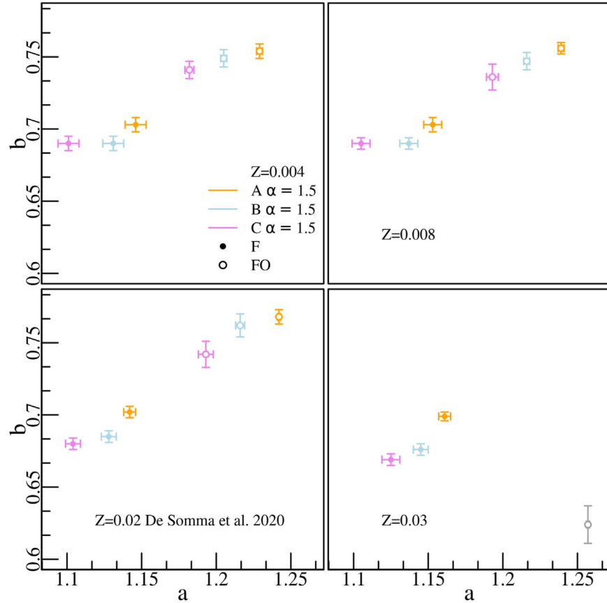
Figure 3. Intercept ( a ) and the slope ( b ) of the fitted F and FO-mode PR relations for Z = 0.004 and Y = 0.25 , Z = 0.008 and Y = 0.25 , Z = 0.02 and Y = 0.28 (taken from De Somma et al. 2020b), and Z = 0.03 and Y = 0.28 for a fixed mixing length parameter of \alpha_{ml} = 1.5 , and as a function of the various assumptions about the ML relation (see the main text and labels for more details).
