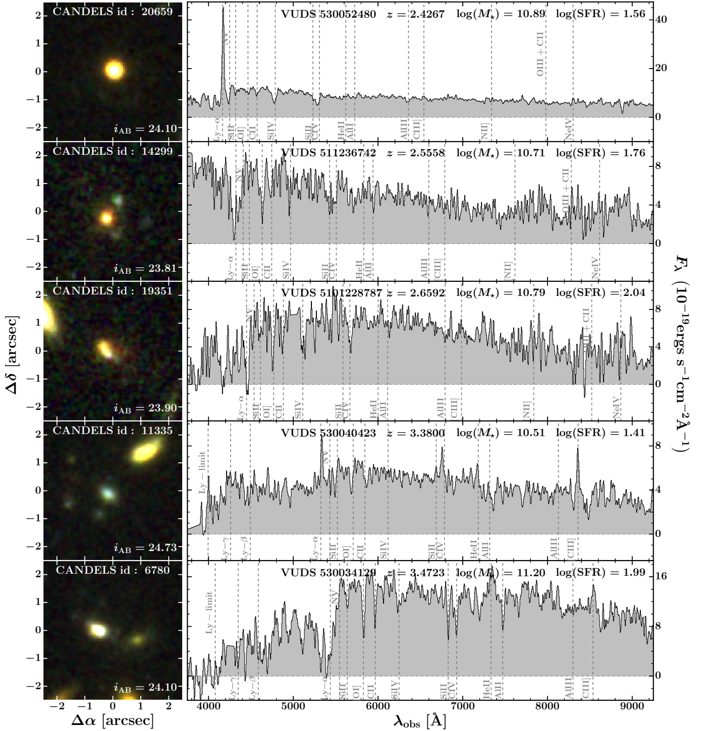
Fig. A.1. HST images, composite of F814W (blue), F125W (green), and F160W (red) from the CANDELS survey (left panels), and observed spectra (right panels) for the ten most massive and strongest star-forming galaxies (see text) in the VUDS-DR1. The CANDELS ID number is indicated in each of the left panels, while the ID, the spectroscopic redshift from VUDS-DR1, and the stellar mass M_* and SFR are indicated for each galaxy in the right panels.
