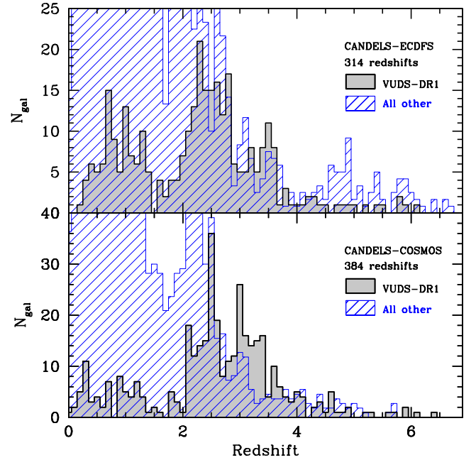
Fig. 3. Redshift distribution of the VUDS-DR1 in the CANDELS-COSMOS (bottom) and in the CANDELS-ECDFS (top) fields. All galaxies with a spectroscopic redshift measurement available in these two fields are presented. The light grey histograms are for VUDS-DR1 sources, while the blue diagonal shaded histograms are for measurements obtained by other surveys.
