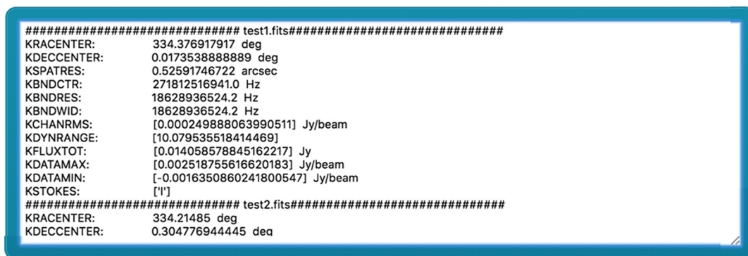
Fig. 3 Example of the KAFE keyword catalog output for a list of images. See the Appendix for the AKF keyword definitions.
