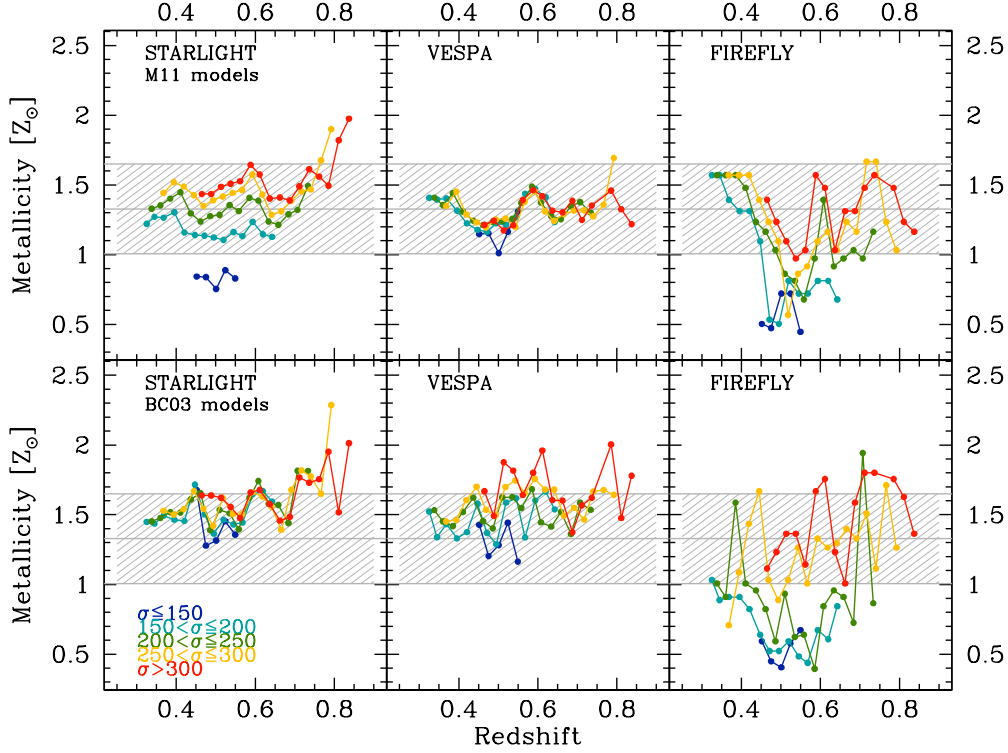
Figure 3. Stellar metallicity estimated from full spectral fitting with STARLIGHT, VESPA and FIREFLY (respectively left, center and right panels), and adopting M11 and BC03 models (respectively upper and lower panels). The grey shaded region represents the mean value, averaged between all models and codes, as discussed in the text.
