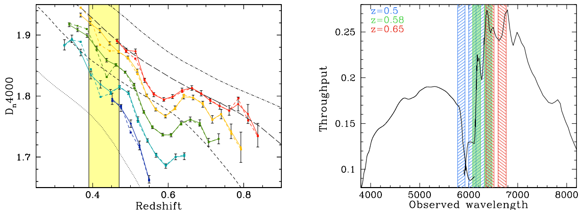
Figure 10. In the left plot is shown the median D_n4000 - z relation before (open points, dotted lines) and after (filled points, solid lines) the sigma clipping correction; the correction is in particular effective around z \sim 0.4 , where the 5577 Å line enters the D_n4000 range. As in figure 5, dashed lines show D_n4000 from models. In the right plot are presented the throughput curves for the red and blue arms of BOSS spectrograph ([53], see also http://www.sdss.org/dr12/algorithms/spectrophotometry/ ) as a function of observed wavelength. The shaded regions with the same colors highlight the left and right bands where D_n4000 is calculated, at three different redshifts ( z = 0.5 in red, z = 0.58 in green, and z = 0.65 in blue) around which the wiggle in the median D_n4000 - z relations is observed, showing that at these redshifts the D_n4000 transits from the blue to the red arm of the spectrograph.
