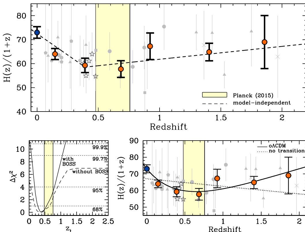
Figure 8. Constraints on the cosmological transition redshift obtained in a model-independent way. In the upper panel are shown the fitted H(z)/(1+z) measurements in grey, with the same coding of figure 6, where the starred symbols are the measurements obtained from this analysis; for this fit we used BC03 measurements for homogeneity with the estimates obtained in literature data. Orange points show the binned values, for illustrative purposes; the analysis is performed on unbinned data. The H_0 value used in this analysis is plotted in blue. The transition from decelerated to accelerated expansion is clearly visible by eye as a turn in the slope of the data. The solid line represents the best fit to the data with a cosmology-independent piecewise linear function. As a comparison, model dependent 2\sigma constraints obtained from Planck (2015) [9] in an open \Lambda CDM cosmology are shown in yellow. In the lower-left panel the effective \Delta\chi^2 is shown as a function of z_t , with and without considering the new BOSS data; the improvement of the statistical significance of the result provided by the new data is clearly evident. In the lower-right panel are presented for comparison the best fits obtained for the \text{o}\Lambda\text{CDM} model and for the model without a transition redshift.
