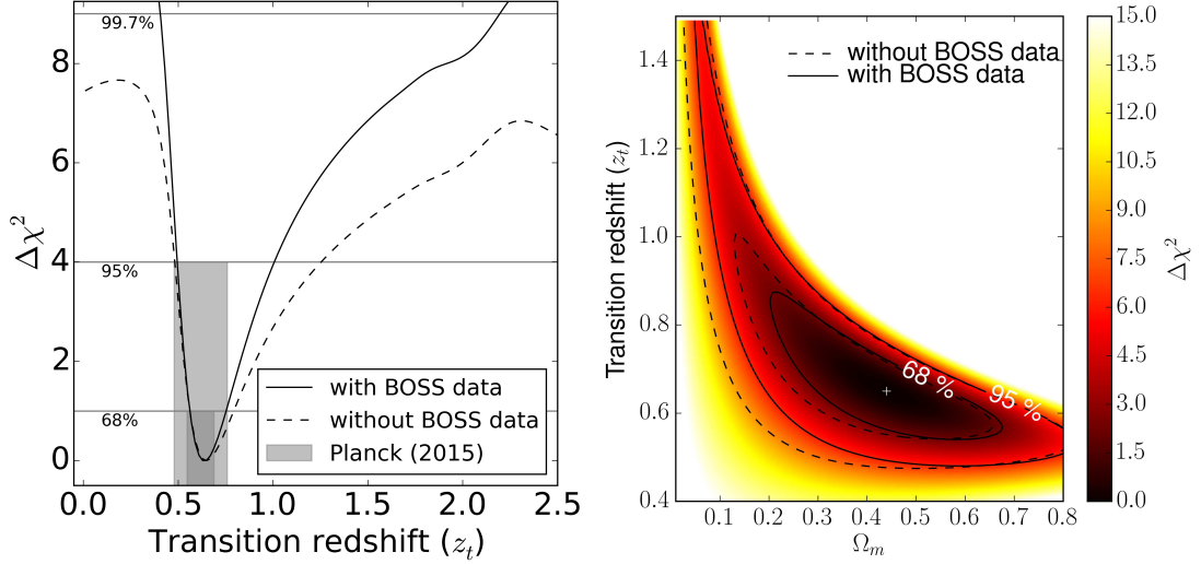
Figure 7. Constraints on the cosmological transition redshift obtained in a \Lambda CDM cosmology. The left panel shows the effective \Delta\chi^2 as a function of z_t . The solid line shows the constraint obtained with the data of Tab. 4, while the dashed line shows the constraint obtained without the values obtained in this work. As a comparison, the grey shaded area represent the 1\sigma and 2\sigma constraints from Planck (2015) for an \Lambda CDM cosmology. In the right panel the 68% and 95% two-dimensional constraints are shown in the \Omega_m - z_t plane, both with and without the new H(z) data obtained in this analysis.
