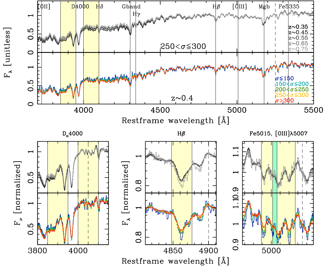
Figure 2. Median stacked spectra as a function of redshift bins and \sigma bins (the upper and lower panels of each plot respectively). The spectra in the upper panels of each plot are extracted at fixed \sigma (grey lines, 250 < \sigma < 300 ), while the spectra in the lower panels are extracted at fixed redshift (colored lines, z \sim 0.4 ). The upper plots show the median spectra. All spectra have been normalized near to the vertical dashed lines; therefore the differences in the upper panels flatten at higher wavelengths, but the steepening of the slope of the continuum with increasing mass and decreasing redshift is evident. This trend may be interpreted in the framework of the “mass-downsizing” scenario, with more massive galaxies being redder and older than less massive ones. The lower plots are zoom-in around three specific absorption features, i.e. D_n4000 , H\beta , and Fe5015 , highlighted in yellow; it is also shown, highlighted in green, the region corresponding to [OIII]\lambda 5007 line.
