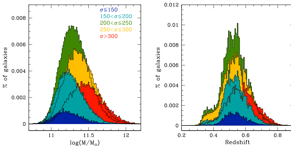
Figure 1. Stellar mass (left panel) and redshift (right panel) distributions, colored by the various velocity dispersion subsamples.
