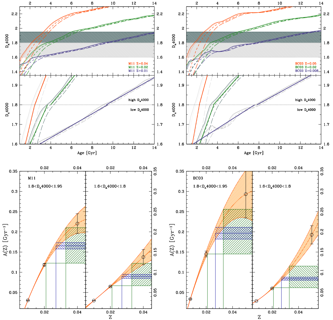
Figure 4. Calibration of the D_n4000 -age relations. Upper plots: D_n4000 -age relation for different EPS models, metallicities and SFH. Left and right panels show M11 and BC03 models, respectively, where the green lines show the relations for solar metallicity, blue for sub-solar and orange for over-solar; lines from solid to dashed represent SFH with progressively higher \tau , from 0.05 to 0.3 Gyr. Lower panel show the linear best fit to each metallicity, in the two D_n4000 ranges discussed in the text. Lower plots: fitted A(SFH, Z/Z_\odot) -metallicity relation for different EPS models. The orange shaded area represent the best fit to the data, shown as black points. The green shaded area represent the total error on A(SFH, Z/Z_\odot) , given the uncertainty on the measured metallicity, while the blue area show the contribution to the error due to SFH.
