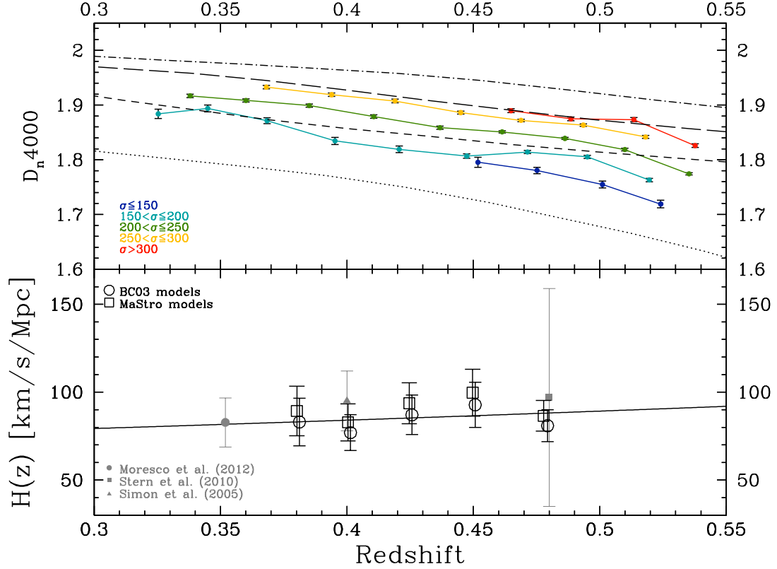
Figure 5. Upper panel: median D_n4000 - z relations obtained for the various velocity dispersion subsamples. The dashed lines show the theoretical D_n4000 - z relations estimated from M11 models (with solar metallicity) for four differed redshifts of formation, respectively 1, 1.5, 2, 2.5 from bottom to top. Lower panel: H(z) measurements obtained with BC03 and M11 models, compared with literature data available in this redshift range [11, 12, 13]. For illustrative purpose, the estimates obtained with BC03 models have been slightly offset in redshift.
