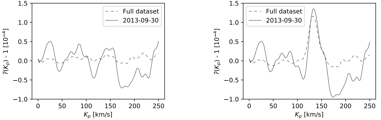
Fig. 7. Left panel : \bar{\tau}(K_p) for the full dataset (dashed line) and the night of 2013 September 30 (solid line). Right panel: same as the left panel, but after the injection of a fake planetary signal with K_p = 132 \text{ km s}^{-1} and \epsilon_{\max} = 10^{-4} .
