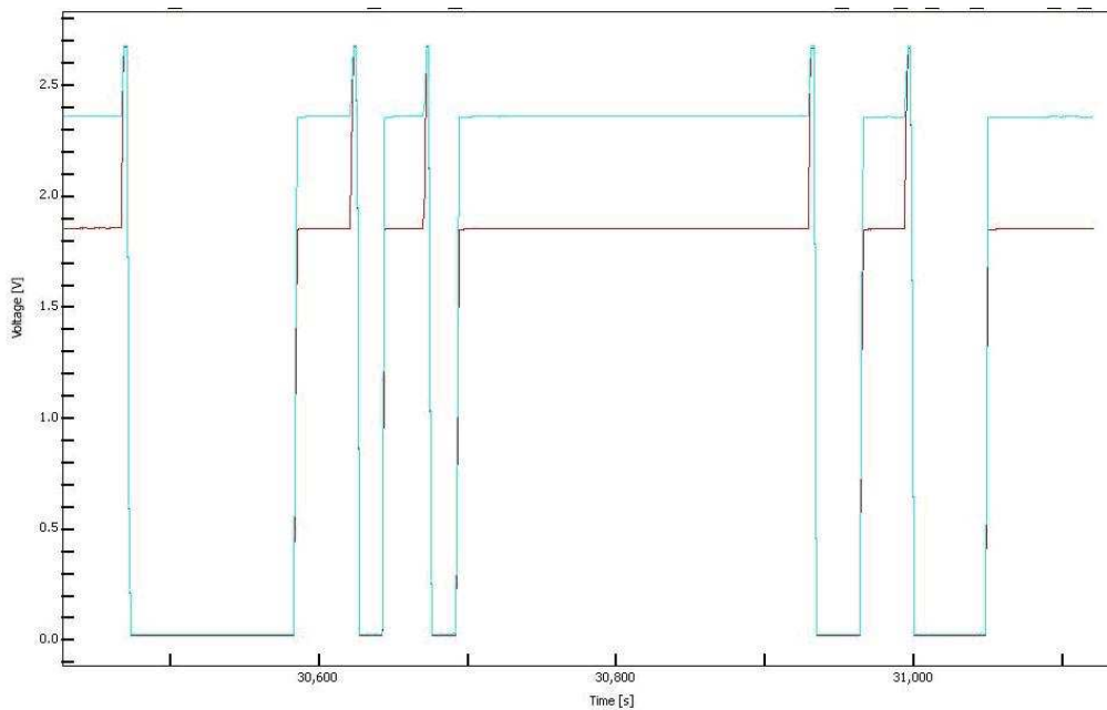
Figure 16: RCA 28 is switched ON-OFF several times using the standard procedure: red and cyan trace represents V_{out} (R0D0) and V_{out} (R0D1), respectively.
