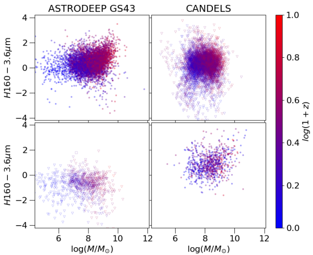
Fig. 11. Compared colour-mass diagrams ( H160-3.6\mu\text{m} vs. stellar mass) of the GS43 and CANDELS catalogues, colour-coded as a function of redshift. Left panels: stellar mass and colour are from the GS43 catalogue; right panels: they are from CANDELS, with photometry from G13 and masses from Santini et al. (2015); in both cases we considered the standard \tau models that include emission lines. Upper panels: sources that in GS43 are detected ( S/N > 1 ) in IRAC CH1 and are upper limits in G13; the lower panels show the opposite.
