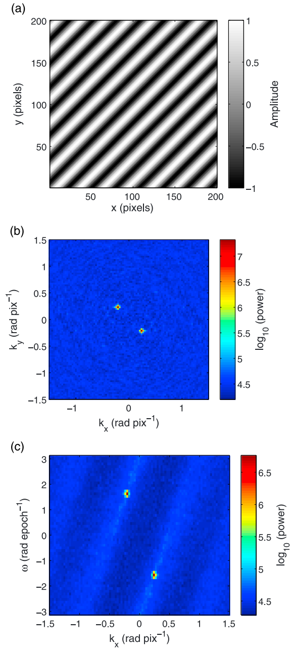
Figure A1. (a) Snapshot of input plane wave for experiment 1, which has a wavelength of 20 pixels and a period of four epochs, and the output power spectrum averaged over (b) \omega and (c) k_y showing a peak at |k| = 0.32 \text{ rad pix}^{-1} , \omega = 1.6 \text{ rad epoch}^{-1} . The diagonal ripples in Figure A1c are features of the response function for data set B, whose sampling distribution was borrowed for this experiment.
