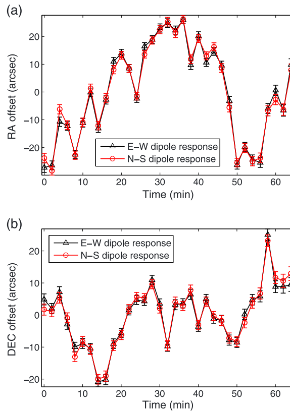
Figure 13. Comparison of the angular offsets of a bright ( 35\sigma ) source between images recorded in the two independent instrumental polarizations, along the (a) RA and (b) Dec directions (these are orthogonal). Error bars indicate the precision associated with Gaussian fitting. The two independent measurements are consistent with one another to within the measurement precision, which is significantly smaller than the amplitude of the position fluctuations themselves.
