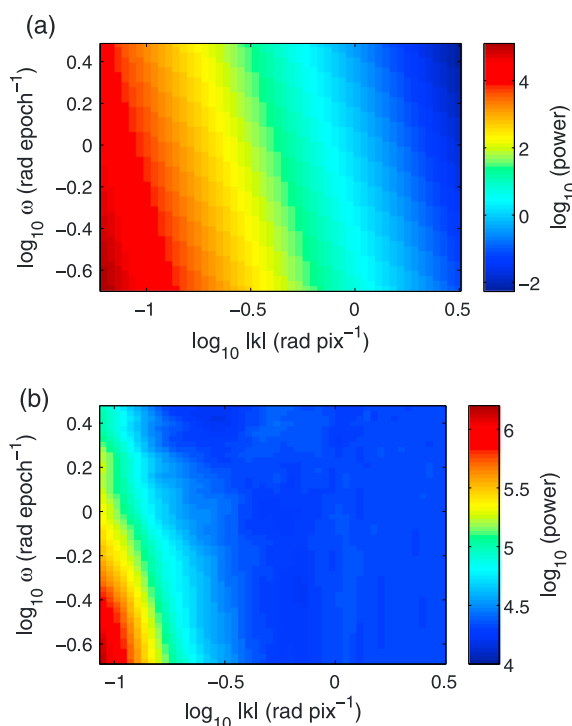
Figure A2. (a) The input power spectrum for experiment 2 and (b) the output power spectrum, shown on logarithmic axes. The output spectrum has been boxcar-smoothed with a 3 \times 3 pixel element with respect to the linear grid. Note the use of logarithmic axes, which are best for visualizing a power law.
