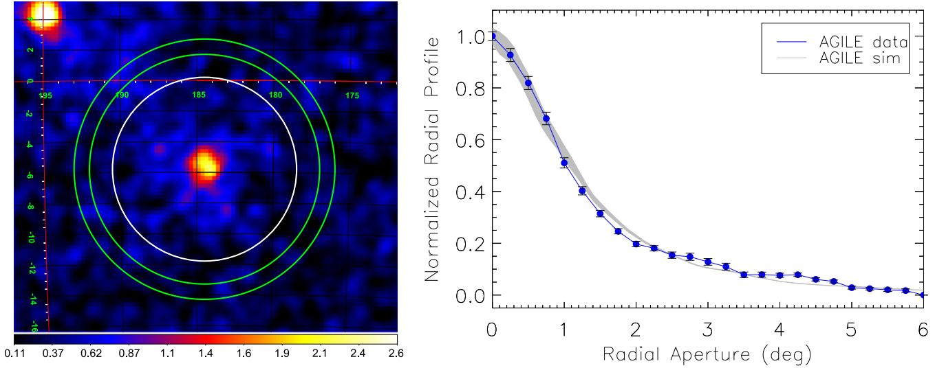
Figure 4. Left panel: AGILE /GRID count map of the Crab system (pulsar + Nebula) for the period 2007-09-23T12:01:05-2007-10-04T12:01:05 in the 100–400 MeV energy band; the white circle shows the maximum aperture ( 6^\circ ) used to produce the radial profile of the source shown in the right panel; green circles show the crown region used to estimate the background emission ( 7^\circ5-8^\circ5 radius). Right panel: average count radial profile: blue data points are the in-flight data, while the gray shaded region shows the profile for the simulated crab system with errors. The counts are normalized to the maximum value of the profile in order to reach 1 at 0^\circ . The source in the upper left corner is Geminga.
