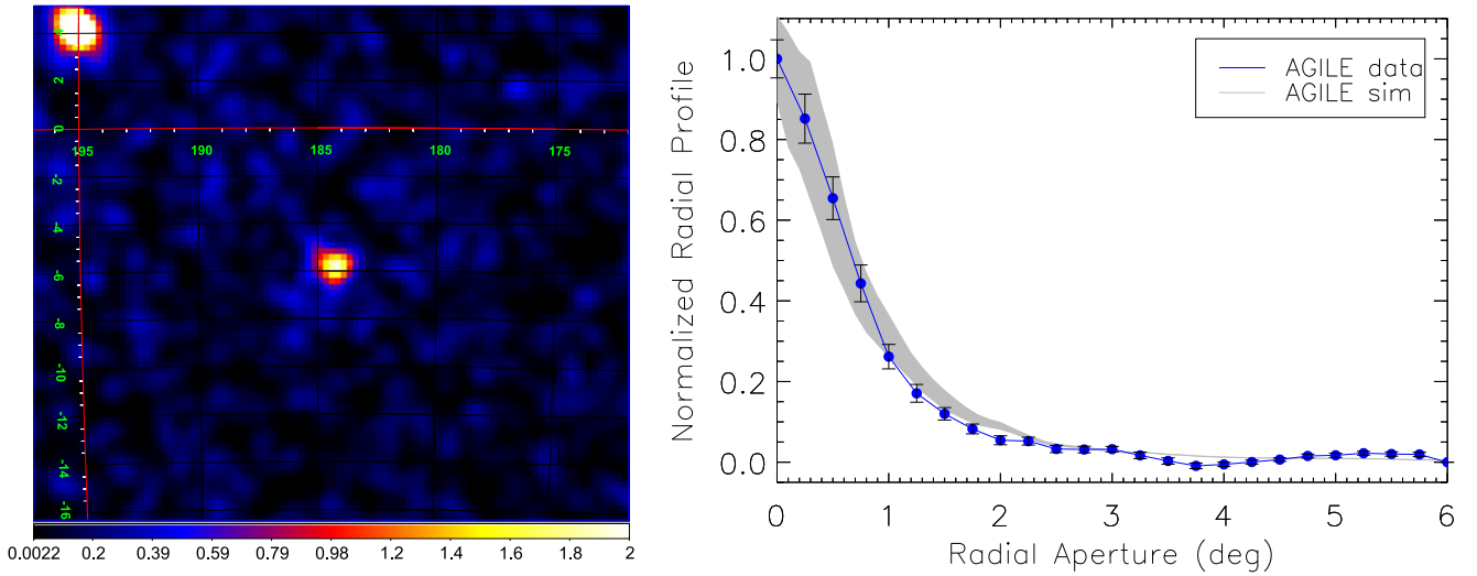
Figure 5. Left panel: AGILE /GRID count map of the Crab system (pulsar + Nebula) in the 400–1000 MeV energy band. Right panel: average count radial profile: blue data points are in-flight data, while the gray shaded region shows the profile of the simulated crab system with errors. The counts are normalized to the maximum value of the profile in order to reach 1 at 0^\circ .
