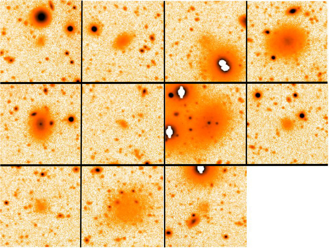
Figure 3. Selected LSB dwarfs in the Virgo-xmmuj1230 field; the box size of each image is \simeq 57 arcsec. The sequence from the top left to the bottom follows the list in Table 1.
