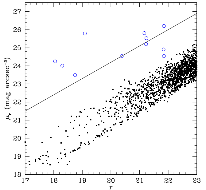
Figure 1. Surface brightness—magnitude relation for the galaxies in the field. Faint sources located in the extended halos of bright galaxies and blended galaxies have been removed from the plot since they have biased photometry. LSB dwarf candidates are shown as blue circles. The continuous line represents an extrapolation to fainter magnitudes of the LSB selection threshold adopted by Rines & Geller (2008).
