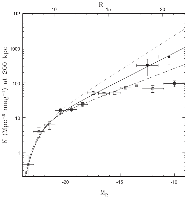
Figure 5. Virgo projected LF normalized at 200 kpc. Filled squares indicate data from the present sample after conversion from AB to the Vega magnitude system by R(\text{Vega}) = r(\text{AB}) - 0.2 . Empty squares are from Trentham & Tully (2002) in the Vega system. The continuous curve represents a Schechter shape with slope \alpha \sim -1.4 and M^* \sim -22.5 . Two faint slopes \alpha \sim -1.3 , -1.5 are also shown for comparison (dashed and dotted lines, respectively).
