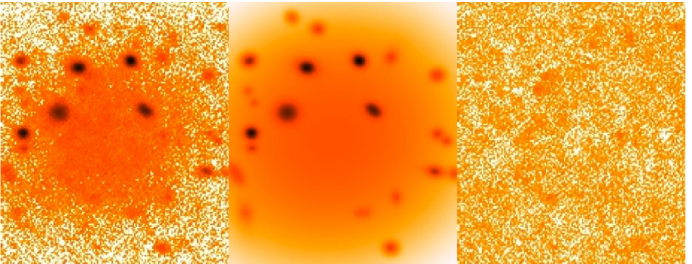
Figure 4. “K” dwarf galaxy. From left to right: observed profile; model profile from Galfit (the brightest background galaxies have been fitted separately); residuals.
