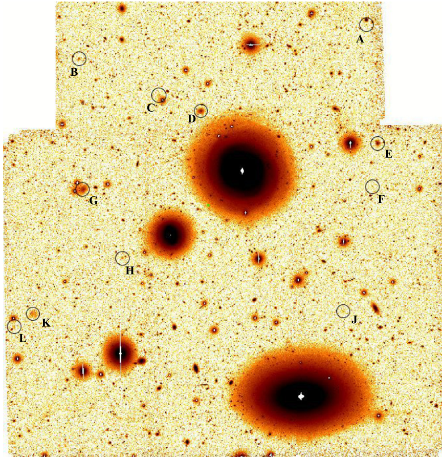
Figure 2. Position of the selected LSB dwarfs in the Virgo-xmmuj1230 LBC field.
