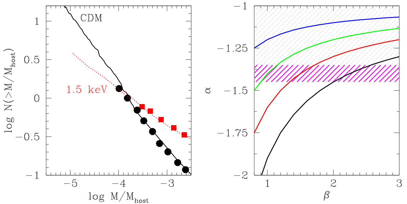
Figure 6. DM model predictions. Left: cumulative mass function vs. satellite over main halo mass ratio predicted by our Monte Carlo model (black and red curves) compared with results derived by Pullen et al. (2014). Black curve and points are for the CDM spectrum and red curve and points for WDM spectrum with m_X = 1.5 keV. Right: luminosity (i.e., stellar mass) function slope \alpha vs. \beta , the slope of the M/L \propto M^{1-\beta} power-law relation. The observed value \alpha = -1.4 \pm 0.05 is shown as a dashed region. Different curves derived from our semi-analytic model are shown for different WDM particle masses and CDM (1, 1.5, 2 keV, and CDM starting from top to bottom). For \beta > 1 then m_X > 1.5 keV if \alpha \simeq -1.4 .
