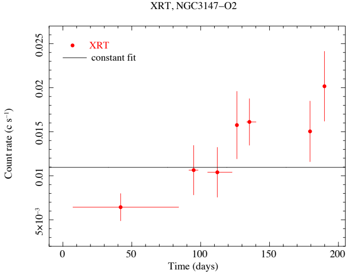
Fig. 7. XRT light curve of the candidate quasar (Flesch 2010) (NGC 3147-O2). The time zero is set to MET = 409627840 s (2013-12-25). The mean rate is 1.10 \times 10^{-2} counts s ^{-1} , \chi^2 = 20.73 (6 d.o.f.) and p = 0.0021 .
