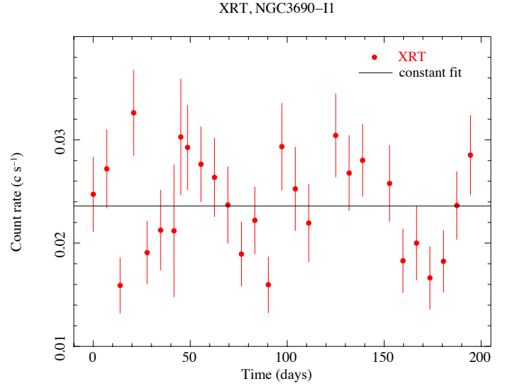
Fig. 8. X-ray radiation detected inside the target galaxy NGC 3690 (NGC 3690-I1). This galaxy is not characterised by an active nucleus, so the radiation is likely generated by a number of X-ray emitters inside the galaxy. The time zero is set to MET = 411013065 s (2014-01-10). The fit performed on the data with a constant function returns a rate of 2.36 \times 10^{-2} counts s ^{-1} , a \chi^2 = 62.85 (35 d.o.f.) and p = 0.0026 .
