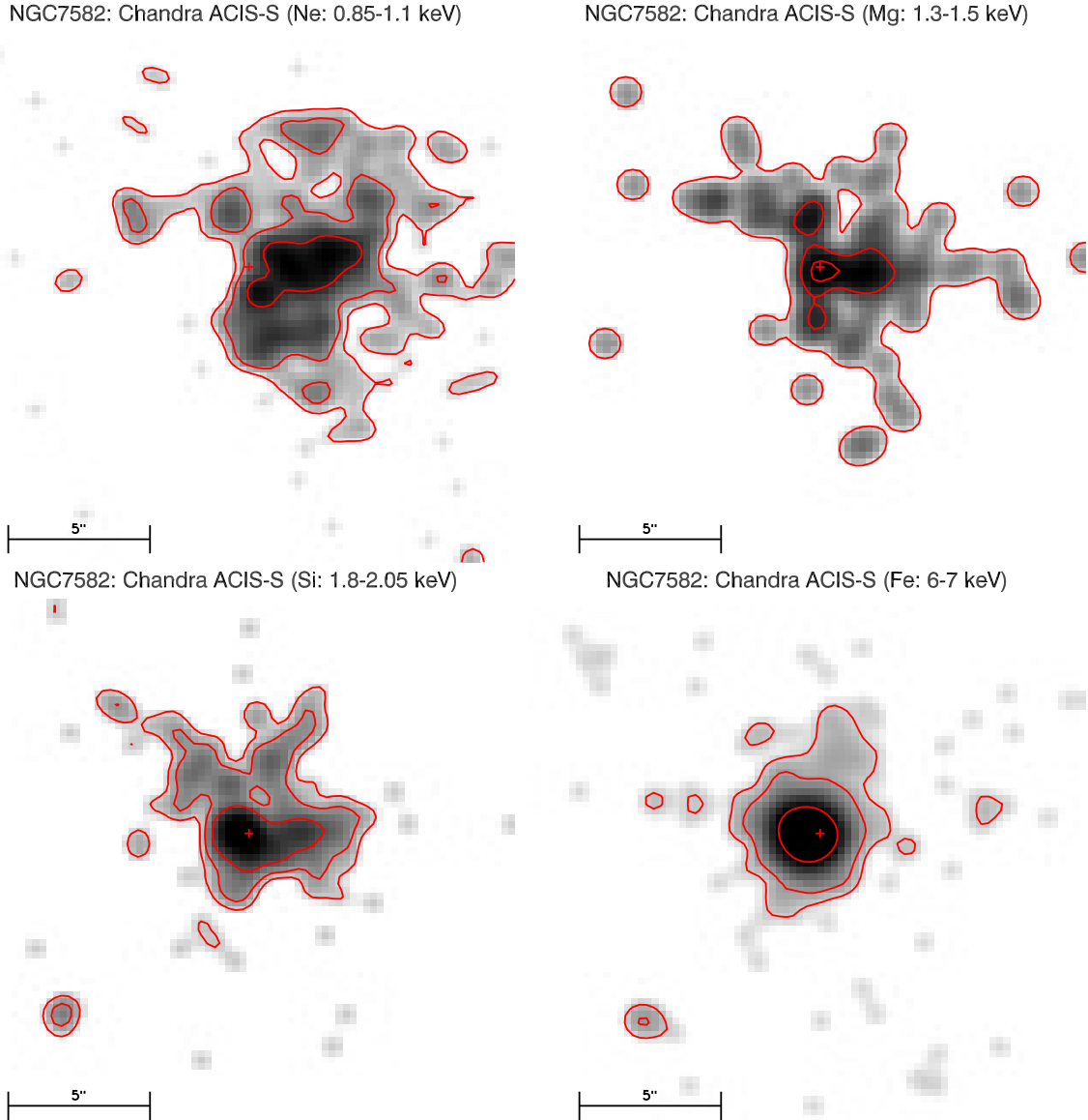
Fig. 6. ACIS-S zeroth order images of NGC 7582 mapping, from top to bottom, the Ne IX-X (upper left panel), the Mg XI-XII (upper right panel), the Si XIII-XIV (lower left panel), and the Fe K \alpha (lower right panel) energy ranges. In all the images the red crosses indicate the coordinates of the nucleus (from NED) and the spatial scale is reported at the bottom (note that for NGC 7582 1'' corresponds to 109 pc). The emission appears to be spatially extended in almost all the energy ranges with a different morphology depending on the energy. The emission is progressively less extended with increasing energy and at the Fe K \alpha emission line it is almost consistent with a point-like source, albeit with a weak elongation in the north direction. The Chandra PSF HEW is 0.5''.
