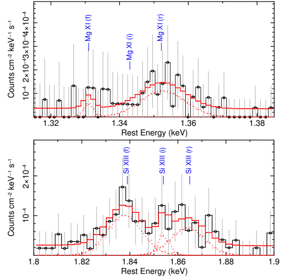
Fig. 4. Zoom into the MEG spectrum at the energy of the Mg XI and Si XIII triplets with the 4096 channels binning (i.e., at FWHM of the spectral resolution). The blue labels indicate the expected position of the forbidden, intercombination, and resonance transitions. The top panel shows the Mg XI region. While there is no evidence of emission at the energy of the forbidden component, the finer binning confirms both the strength and broadening of the resonance emission line. The lower panel shows the Si XIII triplet, where the finer binning confirms both the strength and broadening of the forbidden and resonance emission lines. While it is not statistically required ( \Delta C = 2 ) we also included a Gaussian emission line to account for a possible intercombination component.
