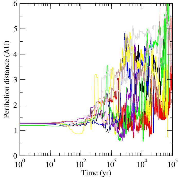
Fig. 1. Evolutions of the perihelion distance of 67P, found by forward integrations of random initial orbits leading into current orbits close to the one of 67P. The time plotted on the abscissa is counted backward from the present. The different colors mark the different examples chosen. We note that these are not clones of 67P, and the recent history of 67P (including the close encounter with Jupiter in 1959) is not reproduced. The focus is on the long-term dynamics, shown in the right part of the diagram. Chaotic divergence of the backward motions sets in, mostly a few centuries ago, due to close encounters with Jupiter. Courtesy Ryszard Gabryszewski.
