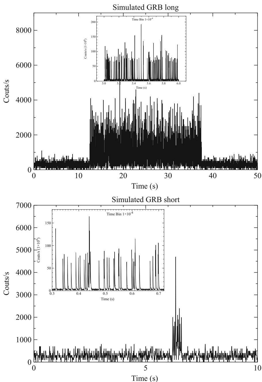
Fig. 1 lightcurves on timescales of 10^{-2} seconds for the synthetic long (top panel) and short (bottom panel) GRBs created following the procedure described in Section 3.2. The insets show a zoom-in of the lightcurves created on shorter timescales ( 10^{-4} seconds) after rescaling the effective area of the equivalent detector up to 100 square meters
