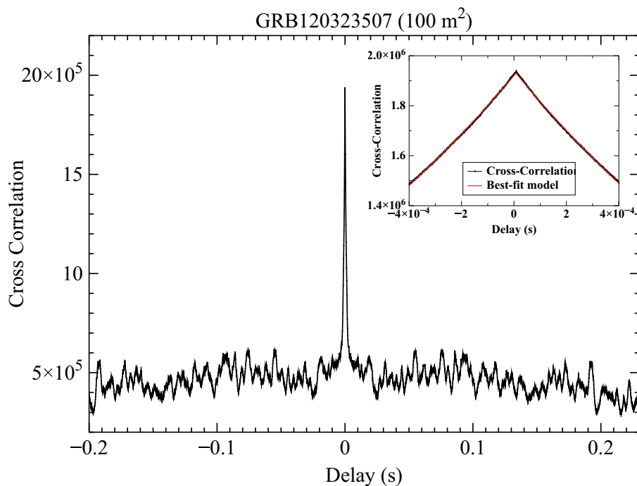
Fig. 3 Cross-correlation function obtained analysing simulated lightcurves obtained from a template generated starting from the Fermi GBM observations of the short GRB 120323507. See text for more details
