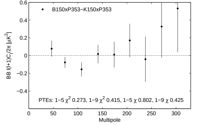
FIG. 4. Differences of B150×P353 and K150×P353 BB cross-spectra. The error bars are the standard deviations of the pairwise differences of signal+noise simulations that share common input skies. The probability to exceed the observed values of \chi^2 and \chi statistics, as evaluated against the simulations, is quoted for bandpower ranges 1–5 ( 20 < \ell < 200 ) and 1–9 ( 20 < \ell < 330 ). There is no evidence that these spectra are statistically incompatible.
