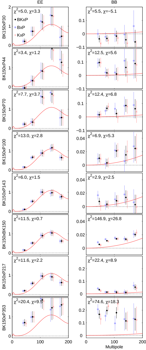
FIG. 3. EE (left column) and BB (right column) cross-spectra between BICEP2/Keck maps and all of the polarized frequencies of Planck . In all cases the quantity plotted is \ell(\ell+1)C_\ell/2\pi in units of \mu\text{K}_{\text{CMB}}^2 , and the red curves show the lensed- \Lambda\text{CDM} expectations. The error bars are the standard deviations of lensed- \Lambda\text{CDM} +noise simulations and hence contain no sample variance on any other component. Also note that the y -axis scales differ from panel to panel in the right column. The \chi^2 and \chi (sum of deviations) versus lensed- \Lambda\text{CDM} for the five bandpowers shown is marked at upper left. There are no additional strong detections of deviation from lensed- \Lambda\text{CDM} over those already shown in Fig. 2 although BK150×P217 shows some evidence of excess.
