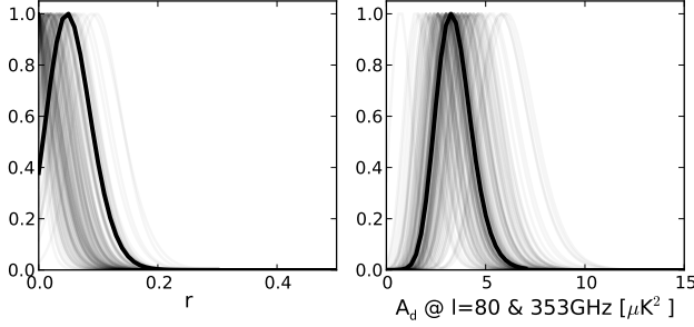
FIG. 10. Likelihoods for r and A_d , using BICEP2/Keck and Planck, as plotted in Fig. 6, overlaid on constraints obtained from realizations of a lensed- \Lambda CDM+noise+dust model with dust power similar to that favored by the real data ( A_d = 3.6 \mu\text{K}^2 ). Half of the r curves peak at zero as expected.
