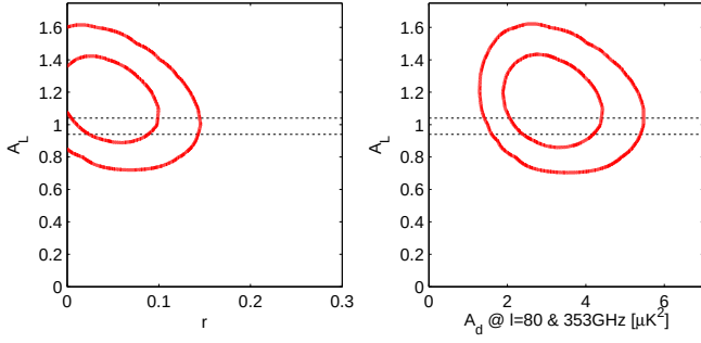
FIG. 9. Likelihood results for a fit allowing the lensing scale factor A_L to float freely and using all nine bandpowers. Marginalizing over r and A_d , we find that A_L = 1.13 \pm 0.18 and A_L = 0 is ruled out with 7.0\sigma significance.
