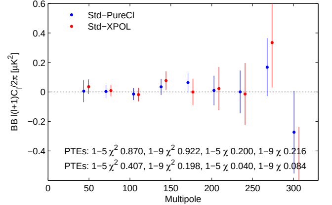
FIG. 5. Differences of B150×P353 BB cross-spectra from the standard power spectrum estimator and alternate estimators. The error bars are the standard deviations of the pairwise differences of signal+noise simulations that share common input skies. The probability to exceed the observed values of \chi^2 and \chi statistics, as evaluated against the simulations, is quoted for bandpower ranges 1–5 ( 20 < \ell < 200 ) and 1–9 ( 20 < \ell < 330 ). We see that the differences of the real spectra are consistent with the differences of the simulations.
