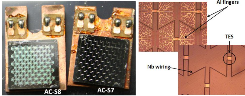
Fig. 3 Left: the AC-S8 and AC-S7 samples. Right: details about the TES, Nb wiring and Al-fingers. (Color figure online).
