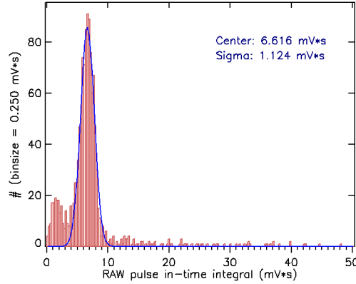
Fig. 6 AC-S7 data pulse in-time integral: raw analysis. A gaussian fit on the main line is overplotted. (Color figure online).
