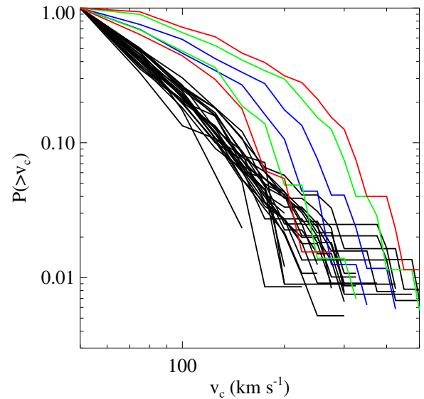
Figure 21. Subhalo velocity functions, i.e., probability distribution functions of subhalos with circular velocities larger than fixed values, of massive galaxy clusters estimated from cosmological simulations and our strong lensing modeling. The simulated (in black) and observed (in color) functions, measured within a two-dimensional aperture of 420 kpc, are normalized to their corresponding values at 50 \text{ km s}^{-1} . The 1\sigma , 2\sigma , and 3\sigma confidence levels, according to the best-fitting 2\text{PIEMD} + 175(+1)\text{dPIE} ( M_T L^{-1} \sim L^{0.2} ) model of MACS 0416, are shown in blue, green, and red, respectively.
