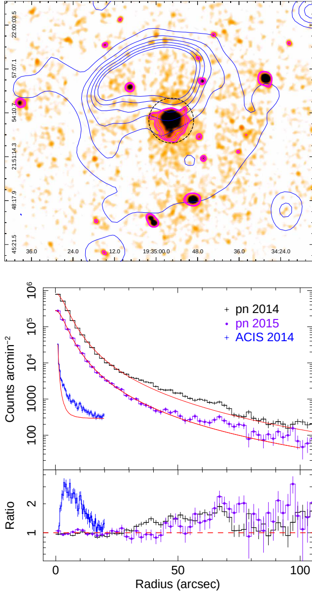
Figure 1. Top: 98ks-long XMM-Newton PN image of the region around SGR J1935+2154; the 1.4 GHz radio map of SNR G57.2+0.8 is also shown (blue contours from the VLA Galactic Plane Survey, Stil et al. 2006; upper image). The XMM-Newton image has been smoothed with a Gaussian function with a radius of 4'' and magenta contours are displayed in order to emphasise the extended emission around SGR J1935+2154. The black dashed circle marks a distance of 90'' from the SGR J1935+2154 position. Bottom: 2014 and 2015 XMM-Newton and Chandra surface brightness (black crosses, purple squares and blue crosses, respectively) as a function of the distance from SGR J1935+2154 compared with their Point Spread Functions (PSF; red lines; lower plot). The ratios between the data and the PSF are plotted in the lowest panel.
