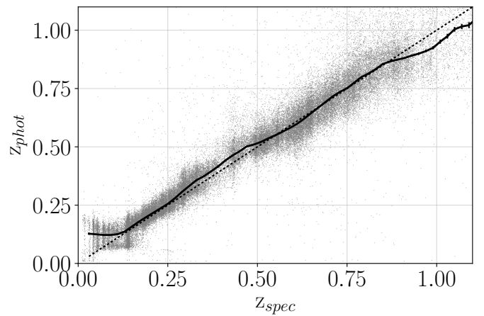
Fig. 3. Relation between the photometric and spectroscopic redshifts, including all objects with a secure spectroscopic measurement (see text). Each grey point represents a galaxy; the black line indicates the bias b(z_{spec}) and its error (only distinguishable at high redshift), which was computed assuming a normal distribution. The dot-dashed black lines indicates z_{phot} = z_{spec} for visualisation purposes.
