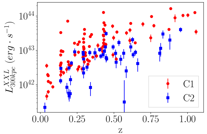
Fig. 1. X-ray luminosity in the [0.5-2] \text{ keV} band computed in a 300kpc aperture as a function of redshift for the cluster sample used in this study. Red points and blue squares represent clusters classified as C1 and C2, respectively (see text).
