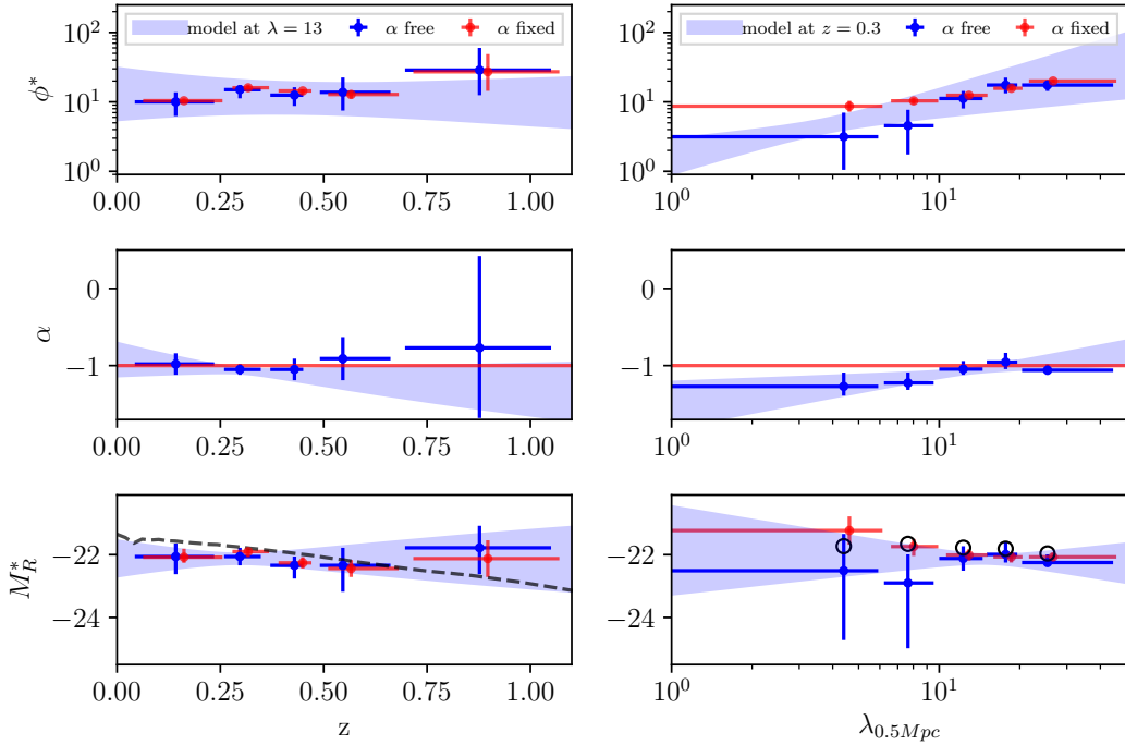
Fig. 13. Parameters of the composite cluster luminosity functions computed in increasing bins of redshift (left) and richness (right). From top to bottom, the plots show the normalisation \phi^* , the faint end slope \alpha , and the characteristic magnitude M_R^* . The vertical error bars indicate the 68% c.i., whereas the horizontal ones reflect the bin size. The blue (red) points indicate the results when the faint end slope is free (fixed). The shaded blue regions show the evolution models we constrained from Eq. 10 at fixed richness (left) and redshift (right). The dashed black line shows a fiducial model for the evolution of M_R^* ; the black circles indicate the model values at the median redshifts of the richness bins.
