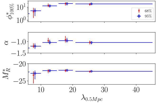
Fig. 18. Evolution of the composite cluster luminosity functions parameters with richness for two different dispersion widths, as indicated in the legend. The vertical error bars indicate 68% c.i., whereas the horizontal ones reflect the bin sizes. The points have been slightly shifted in richness for clarity.
