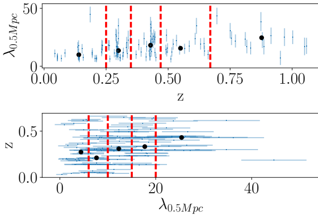
Fig. 11. Illustration of the CLF bin limits. Measurements for individual clusters are represented by the grey error bars. Bin delimitations are indicated by the red dashed lines. Top: Richness in 0.5Mpc as a function of redshift, with a minimum richness of 6. The black dots indicate the median values of the richness in each redshift bin. Bottom: Redshift as a function of the richness in 0.5Mpc, with a maximum redshift of 0.67. The black dots indicate the median redshift value in each richness bin.
