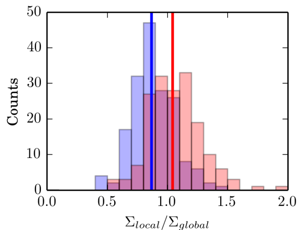
Fig. 7. Histogram of the ratio between local and global background galaxy number densities. Global background refer to the whole CFHTLS W1 field, whereas local backgrounds refer to annuli of 3 to 5 Mpc centred on the X-ray cluster positions. The distribution of the ratio when structures are discarded from (taken into account in) the local background fields is shown in blue (red). The solid lines indicate the median values of the ratios.
