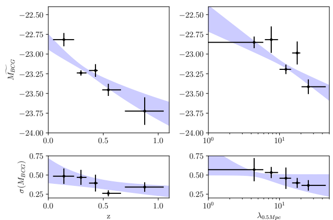
Fig. 14. Parameters of the brightest cluster galaxy (BCG) magnitude distributions, computed in increasing bins of redshift (left) and richness (right). Top: Median BCG magnitude. Bottom: Symmetrised scatter of the BCG distributions around the median values. The shaded blue regions show the evolution models we constrained from Eq. 10, at fixed richness (left) and redshift (right). The vertical error bars indicate the 68% c.i. obtained from bootstrap, whereas the horizontal error bars reflect the bin sizes.
