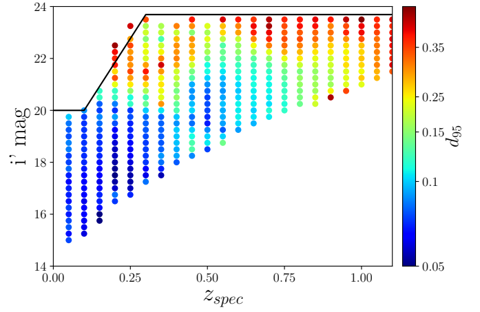
Fig. 5. Photometric redshift dispersion d_{95} , computed as the 95th percentile of |z_{\text{phot}} - z_{\text{spec}} - b(z_{\text{spec}})| in the (z, i' \text{mag}) plane. The dots indicate the centres of the \Delta(z, i' \text{mag}) = 0.1 \times 0.5 cells used to compute the dispersion (if they contain at least 30 objects). The continuous black line shows the limiting magnitude we impose for the rest of the study.
