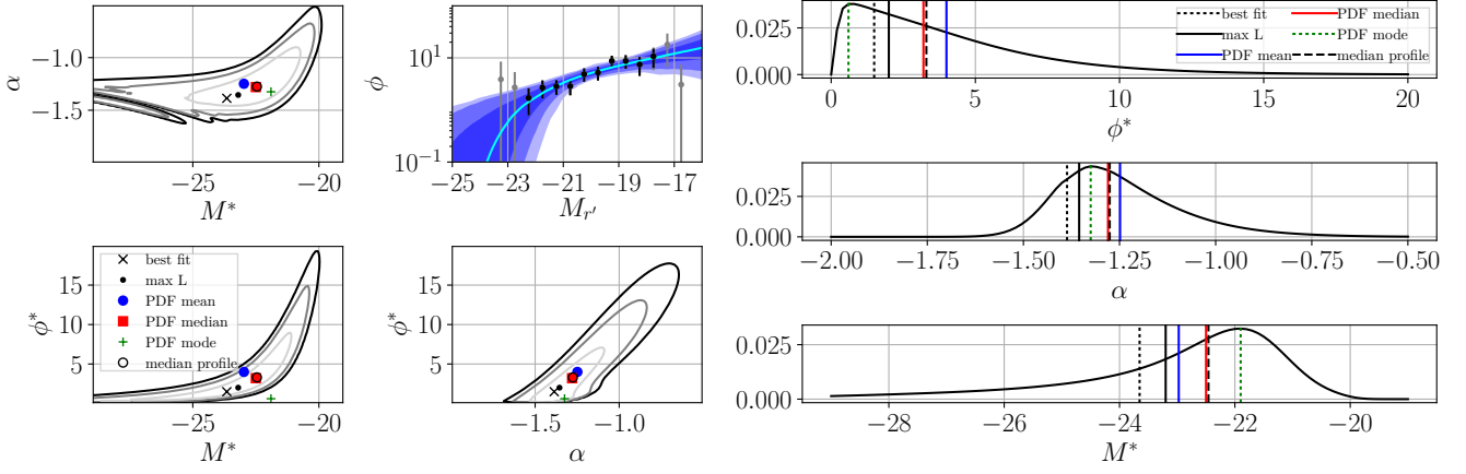
Fig. 16. Illustration of the composite luminosity function fitting procedure as in Figure 15, but for a sample of 26 poor clusters (lowest richness sample in Section 5). In this sample the different statistical estimators give distinguishable values.
