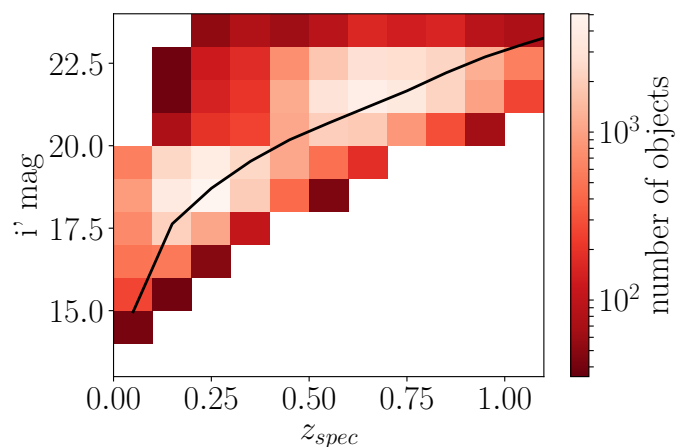
Fig. 2. Number of objects with high quality spectroscopic measurements as a function of spectroscopic redshift and magnitude in the i' band. The black line represents a fiducial evolution model for m^* .
