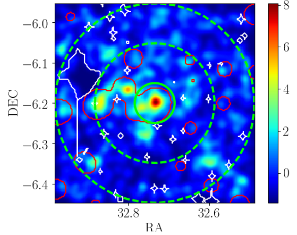
Fig. 6. Example of a density map of a cluster 10 \times 10 \text{ Mpc}^2 field, constructed using a Gaussian kernel of width \sigma = 0.1875 \text{ Mpc} . The colourbar reflects the signal-to-noise ratio. Only galaxies with m < m^* + 3 (or L > 0.06L^* ) are selected and the photometric redshift width depends on the galaxy magnitudes and is taken to ensure 68% completeness. The red contours indicate the structures detected by WAZP, and the white ones show the masked regions. The green inner circle shows 1 Mpc around the cluster X-ray centre and the dashed green lines delineate the local background field from 3 to 5 Mpc. NB: We can see that this cluster is part of a superstructure.
