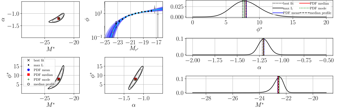
Fig. 15. Illustration of the composite luminosity function fitting procedure for a sample of 121 clusters (general sample in Section 5). Left panels: 2D marginalised likelihoods of the Schechter fit parameters, and associated luminosity profile. The contours show the 68%, 95%, and 99% levels, and the different statistical values are indicated in the legend. Top left: (\alpha, M^*) marginalised over \phi^* ; Top right: Posterior CLF shape, the data points are shown in grey and black, the median profile is drawn in cyan, and the blue shaded regions indicate the 68%, 95%, and 99% c.i.; Bottom left: (\phi^*, M^*) marginalised on \alpha ; Bottom right: (\phi^*, \alpha) marginalised on M^* . Right panels: Probability density functions of the Schechter fit parameters after marginalisation. The lines show the different statistical values, as indicated in the legend. In this sample the different statistical estimators give indistinguishable values.
