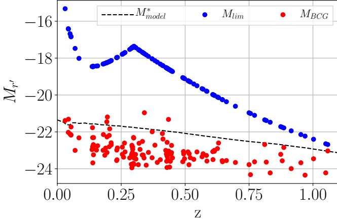
Fig. 8. Redshift evolution of the luminosity range in which the LF are fitted. The red dots show the absolute magnitude of the BCGs of each cluster, whereas the blue ones indicate the limiting magnitude we imposed. A fiducial model (see end of Introduction) for the evolution of M^* is indicated by the black dashed line for comparison.
