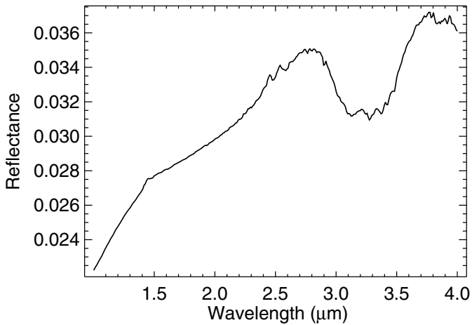
Fig. 3. Spectrum of Dark Terrain unit that corresponds to the average spectrum of the comet's surface.
