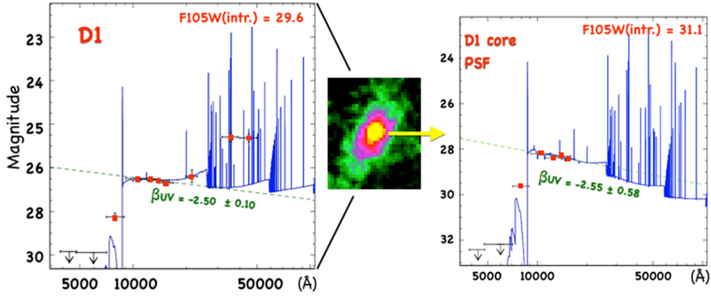
Figure 6. The best SED-fit solutions for D1 (left) and for the core of D1 (right) are shown. Only the HST photometry is shown for the core and no VLT/Ks-band or Spitzer /IRAC magnitudes have been extracted. This comparison shows a first-order consistency among the core and the full D1 object, for which very similar ultraviolet slopes ( \beta_{UV} ) are derived. In the middle, the F105W image of D1 and its core (highlighted in yellow) are shown.
