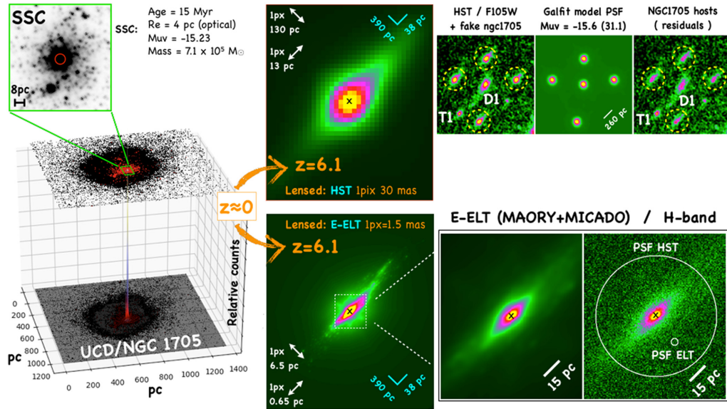
Figure 10. SKYLENS simulation of the ultracompact dwarf galaxy NGC 1705 hosting its SSC. In the left-hand panels, the WFC3/F275W image of the galaxy is shown in 3D and 2D with highlighted the prominent UV emission of the SSC (top-left inset). The main properties of the SSC are also reported. In the top-right panels (from left to right): the modelled noiseless dwarf at the HST resolution lensed at z = 6.143 in the F105W band (the pixel scales are indicated along radial/tangential directions); the same model added to the F105W image in four positions (dashed yellow circles); the GALFIT models of the core of NGC 1705 (see the text for details); the subtracted PSF models of the previous two images, showing the unresolved core of the dwarf dominated by the SSC (the position of the SSC is marked with a black cross in the modelled image). In the bottom panels, the same simulation is shown adopting the MAORY + MICADO PSF in the MCAO narrow field mode. The bottom-right panels show the zoomed region in which the physical scale and the two PSFs ( HST and MICADO + MAORY) are indicated.
