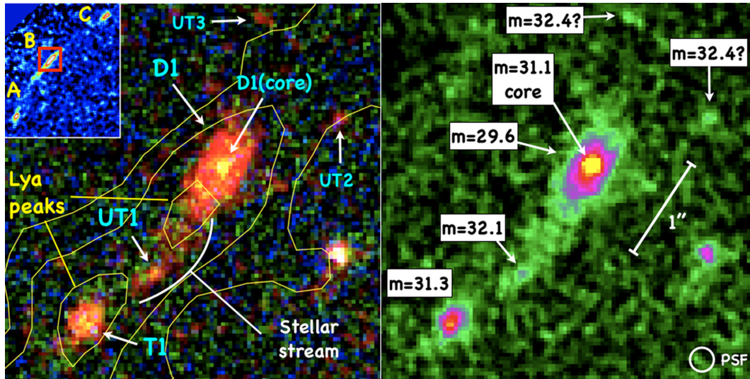
Figure 2. Colour composite (left) and the WFC3/ F105W image (right) of the field under study containing the sources D1 and T1. This region corresponds to the red square in the top-left inset which shows the extended Ly \alpha arc from MUSE (see Fig. 1). Sources are labelled (left), along with their de-lensed F105W magnitudes (right). Note the prominent symmetric core of D1 despite the large tangential magnification and the presence of a stellar stream possibly connecting D1 and T1, also including a star-forming knot, dubbed UT1. Other faint knots are shown, UT2 and UT3, with de-lensed magnitudes fainter than 32. The HST F105W PSF is shown in the bottom right.
