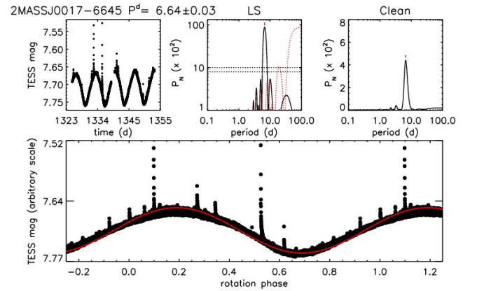
Fig. A.4: Photometric time sequence and periodogram for 2MASSJ0017-6645
