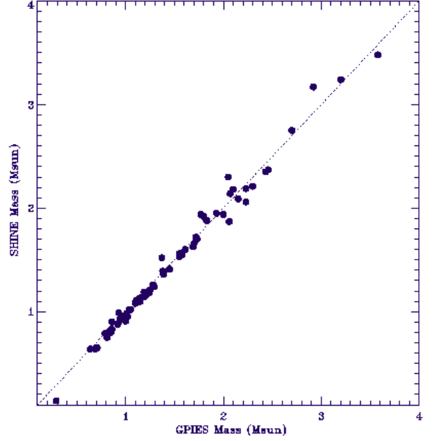
Fig. 10: Comparison of stellar masses derived in the present work and in Nielsen et al. (2019).
