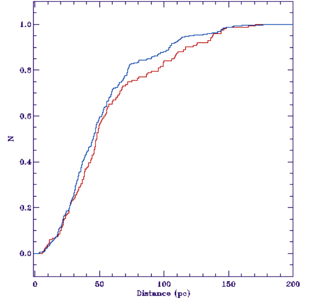
Fig. 6: Cumulative distribution of distance for the stars in our sample (red line) and that of Nielsen et al. (2019) (blue line).
