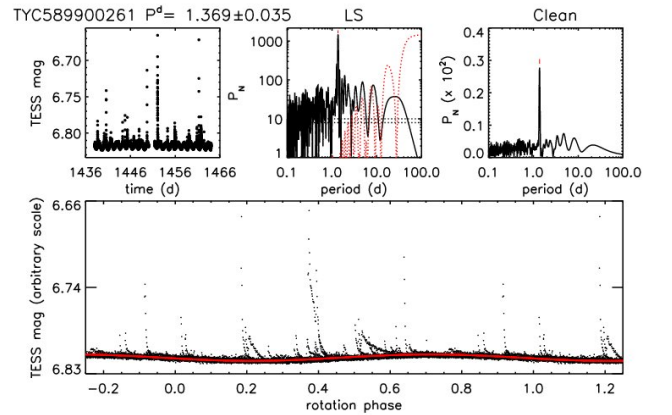
Fig. A.24: Photometric time sequence and periodogram for TYC 5899-0026-1
