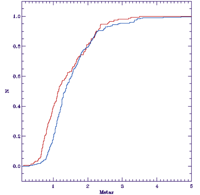
Fig. 7: Cumulative distribution of masses for the stars in our sample (red line) and that of Nielsen et al. (2019) (blue line).
