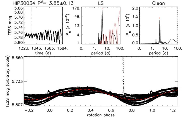
Fig. A.32: Photometric time sequence and periodogram for HIP 30034
