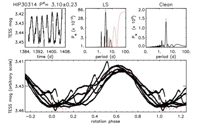
Fig. A.33: Photometric time sequence and periodogram for HIP 30314
