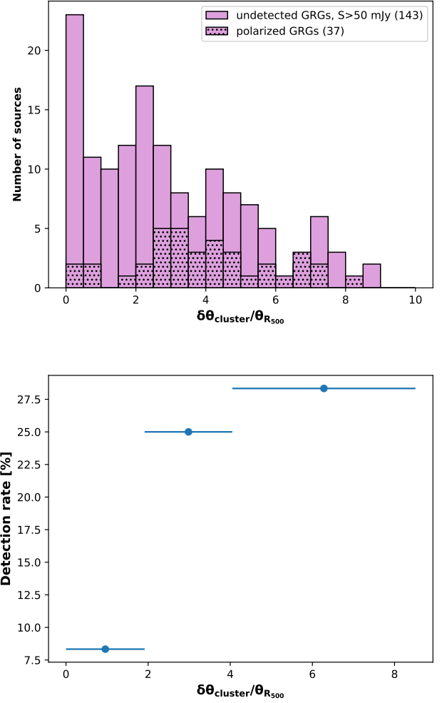
Fig. 7. Distribution of minimum distance from the closest foreground cluster for detected and undetected sources in polarization (top panel), and detection rate as function of the minimum distance from foreground clusters (bottom panel). The widths of the bins are computed to contain the same total number of sources (i.e., 60). Markers are positioned at center of each bin and the error bars show the width of the bins.
