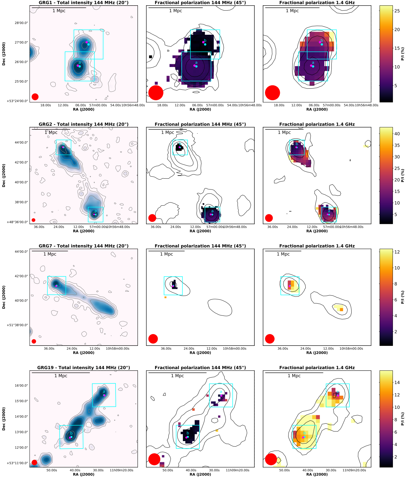
Fig. A.1. Images of the GRGs detected in polarization. Left: LoTSS total intensity image at 20" resolution with contours overlaid. Contours start at 3\sigma noise level and are spaced by a factor of four (with \sigma ranging between 0.09 and 0.9 mJy/beam). Center: LoTSS fractional polarization at 45" resolution with total intensity contours overlaid. Contours start at 3\sigma noise level and are spaced by a factor of four (with \sigma ranging between 0.1 and 8 mJy/beam). Only pixels above the 8\sigma_{QU} detection threshold in polarization are shown (except for GRG 78, for which the threshold is at 7 times \sigma_{QU} , and GRG 80 and GRG 87, for which it is 6\sigma_{QU} ). Right: NVSS fractional polarization with total intensity contours overlaid. Contours start at 3\sigma noise level and are spaced by a factor of four (with \sigma ranging between 0.2 and 0.7 mJy/beam). Only pixels with signal-to-noise higher than three in polarization are shown. The color scale and limits are the same in both P/I images for each source. The cyan squares mark the component detected at 20", cyan points mark the peak of polarized intensity at 20" (RM and fractional polarization values at this position are listed in Tab. 2 and Tab. 3) while magenta points mark the position where we computed the depolarization factors. Letters mark the two components listed in Tab. 2 for double-lobed detected sources.
