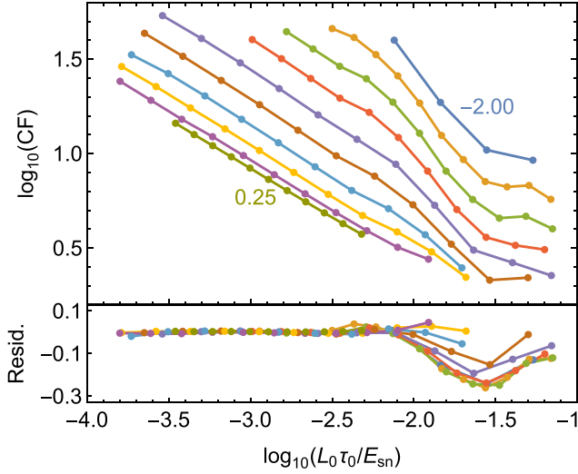
Figure 10. The upper panel gives \log_{10}CF as a function of L_0/L_{ch} , computed for all our models. Each line refers to a given value of \tau_0 , starting from -2.00 (top right) to 0.25 (bottom left), and each dot represents a single model. It is apparent that, for \log_{10}(L_0\tau_0/E_{sn}) \lesssim -2.5 the trend are almost linear. In the text we give an approximating function for this region, and the lower panel displays the residuals after subtracting this function. In the higher energy regime, the most noticeable displacements are: one small bump in the positive direction, at \log_{10}(L_0\tau_0/E_{sn}) \sim -2.4 (actually, near to the value above the first reflected shock reaches the PWN); and another, more prominent, in the negative direction around -1.6 (near the value above which also a second reflected shock appears).
