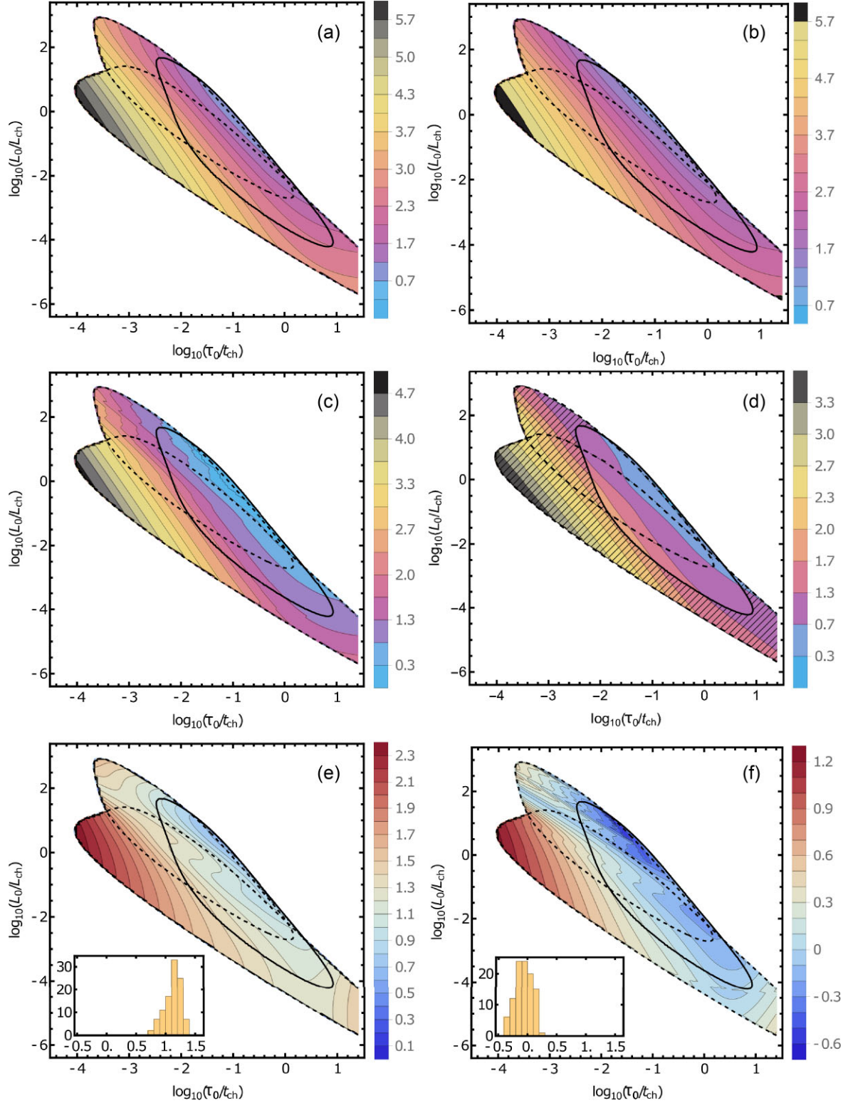
Figure 15. Maps of \log_{10}CF in the parameter space, respectively, using a thin-shell model with P_{outer} = P_{Sedov} (panel A); with P_{outer} \simeq 0.23 \rho_0 V_{FS}^2 (panel B); using our prescription for P_{outer} (panel C); or with using our interpolating formula to our Lagrangian models (panel D). Black contours mark the position of the different populations described in Fig. 1 (ours in solid). Numerical values of \log_{10}CF can be inferred in each panel by the respective vertical color bar (note that the scale is different for different plots). The bottom-row panels show the \log_{10}CF deviations with respect to the results of the numerical simulations, both for P_{outer} = P_{Sedov} (Panel E), and for our prescription for P_{outer} (Panel F). The ratio of the two maps is given in logarithmic scale and also in these cases numerical values can be derived from the vertical color bar. The inset are the histogram of the logarithmic ratios evaluated at the points of our Lagrangian models (they show a lower spread than the associated image because the former one refers to a smaller region).
