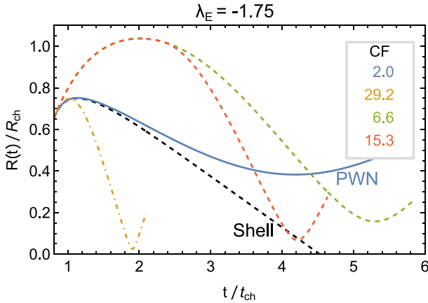
Figure A2. In this figure, we show the evolution of the PWN (solid line, in blue) or shell (dotted line, in black) up to the first compression during reverberation, for the model \lambda_E = -1.75 . For the PWN we have used \log_{10}(\tau_0/t_{ch}) = -1.0 , while the outer pressure is given by the formulas in Appendix C. The dotted–dashed line corresponds to the thin-shell model with PWN + SNR computed considering for the outer pressure P_{Sedov} from equation (26). Dashed lines indeed refer to the case with the outer pressure extrapolated from that at the RS (see equation 27). In the box on the right side of the image, we report the CF as computed from the different models.
