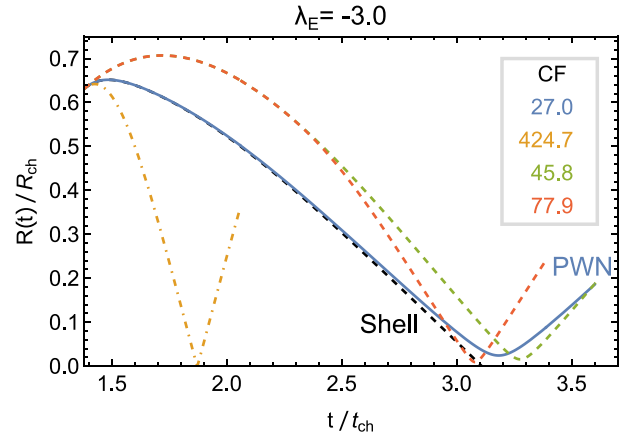
Figure A3. Same as in Fig. A2, but for the model \lambda_E = -3.0 . Again we have used for the PWN \log_{10}(\tau_0/t_{ch}) = -1.0 . Colours and line styles have the same meanings as in the previous figure.
