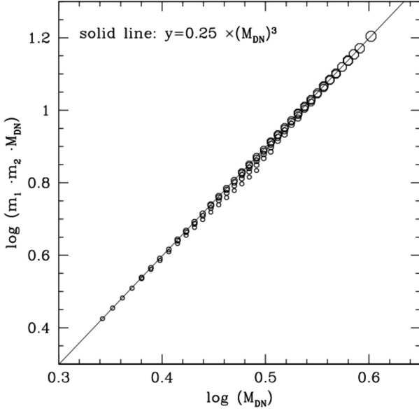
Figure 1. The mass-dependent term in equation (2) is plotted as a function of the total mass of the binary, for m_1 and m_2 ( \leq m_1 ) ranging from 1.1 to 2 M_\odot . Larger symbols refer to higher values of the primary mass. The solid line represents a good approximation to this term.
