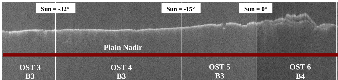
Fig. 3.3.1 (MARSIS Radar gram, first Tx Bands)
