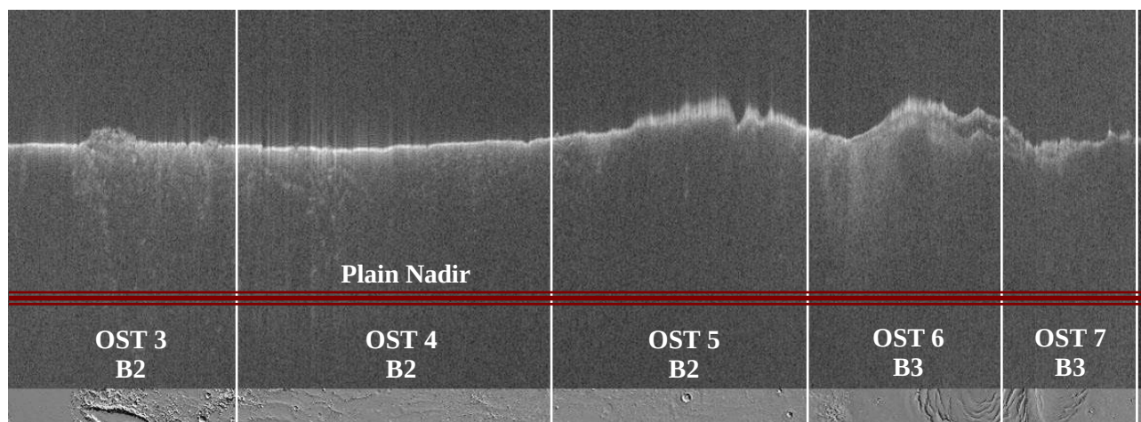
Fig. 3.1.2 (MARSIS Radargram, second Tx Bands)
