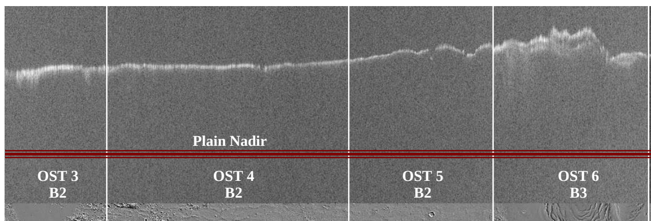
Fig. 3.3.2 (MARSIS Radargram, first Tx Bands)
