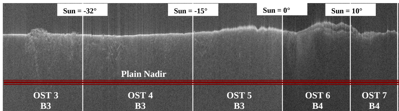
Fig. 3.1.1 (MARSIS Radargram, first Tx Bands)
