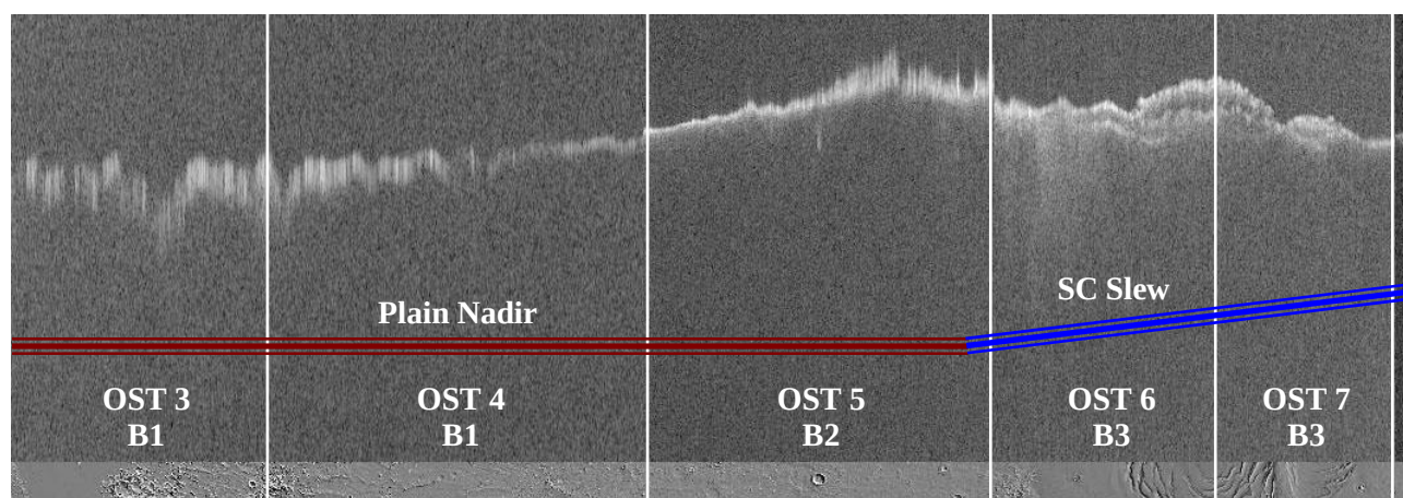
Fig. 3.2.2 (MARSIS Radargram, first Tx Bands)
