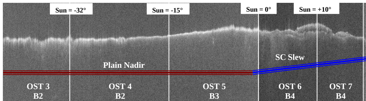
Fig. 3.2.1 (MARSIS Radargram, first Tx Bands)
