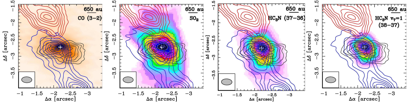
Fig. 8. A zoom on the envelope showing the CO (3–2) outflow lobes indicated in blue and red contours, the \text{CH}_3\text{OH } v_l = 1 line in black contours. The background shows the dust continuum, and moment 0 maps calculated over a velocity range of -55 to -35 \text{km s}^{-1} of \text{SO}_2 , \text{HC}_3\text{N } (J=37-36) , and \text{HC}_3\text{N } v_7 = 1 ( J=38-37 ) from left to right, respectively. White cross marks the position of the dust continuum peak. The beam of the CO ( J=3-2 ) data is shown in the lower left corner.
