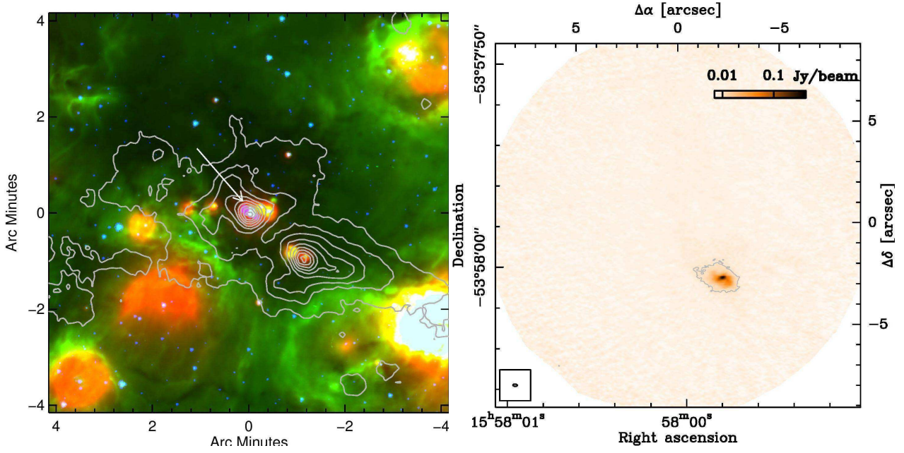
Fig. 1. Overview of the region centred on \ell=+328.2551 , b=-0.5321 in Galactic coordinates. Left: The three-color composite image is from the Spitzer /GLIMPSE (Benjamin et al. 2003) and MIPSAL (Carey et al. 2009) surveys (blue: 4.5\mu\text{m} , green: 8\mu\text{m} , red: 24\mu\text{m} ) and is shown in Galactic coordinates. The contours show the 870\mu\text{m} continuum emission from the ATLASGAL survey (Schuller et al. 2009; Csengeri et al. 2014). The arrow marks the dust continuum peak of the targeted clump. Right: Line-free continuum emission imaged at 345 GHz with the ALMA 12m array. The color scale is linear from -3\sigma to 120\sigma . The contour shows the 7\sigma level. The FWHM size of the synthesised beam is shown in the lower left corner.
