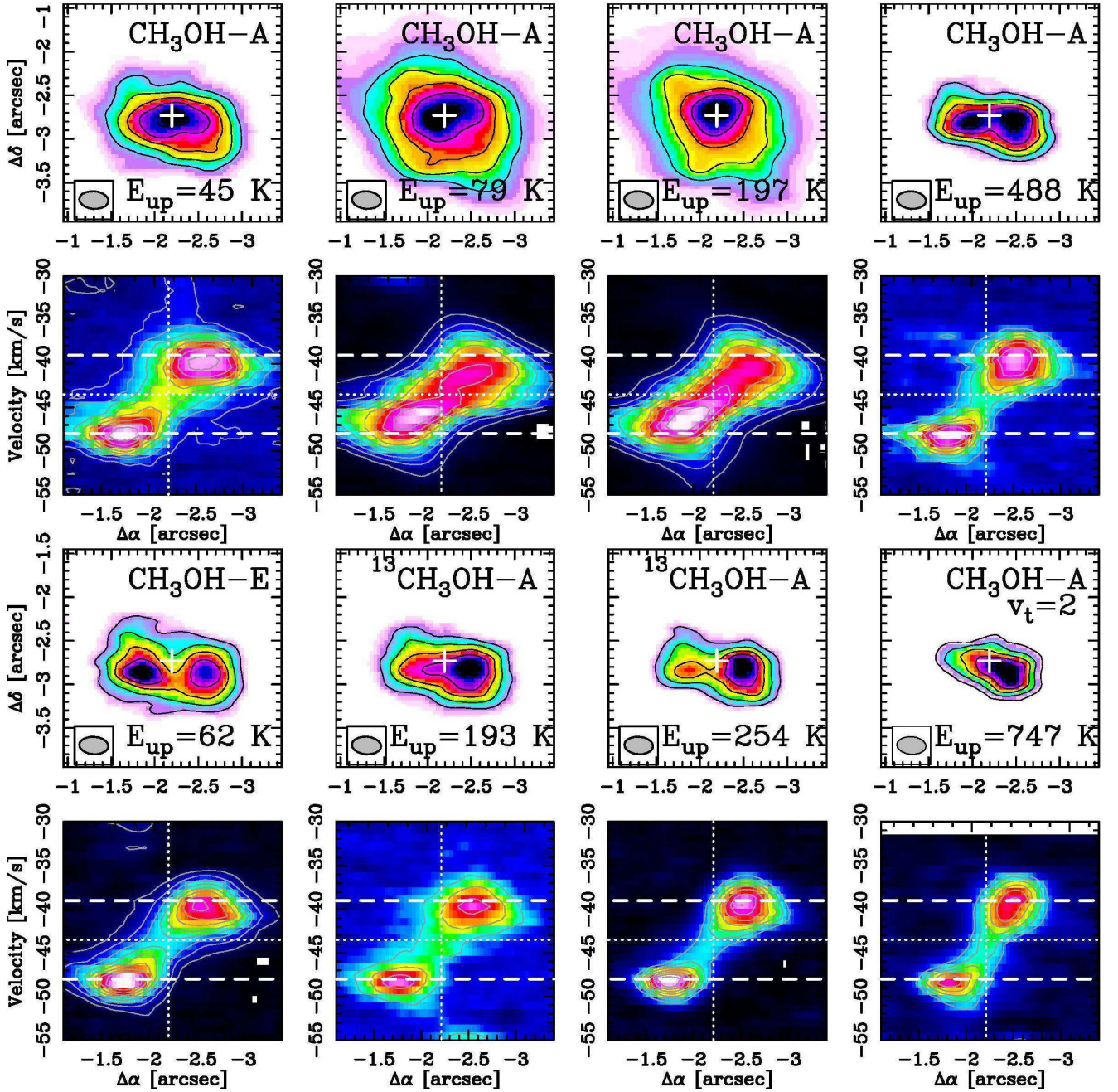
Fig. 5. CH 3 OH 0th moment map and position velocity diagrams for the transitions listed in Table 2. The top row shows the 0th moment map calculated over a velocity range of [-55; -30] km s -1 , contours start at 30% of the peak and increase by 15%. White cross marks the position of the continuum peak. The beam is shown in the lower left corner. The symmetry of the methanol molecule is labeled on each panel, as well as the upper level energy of the transition. The subsequent row shows the position velocity map along the \Delta\alpha axis and averaged over the shown extent of the cube corresponding to \sim 2.5'' . The right-ascension offset of the continuum peak and the v_{\text{lsr}} velocity of the source are marked as white dotted line. Dashed lines show the v_{\text{lsr}} \pm 4.5 km s -1 corresponding to the peak velocity of the CH 3 OH spots.
