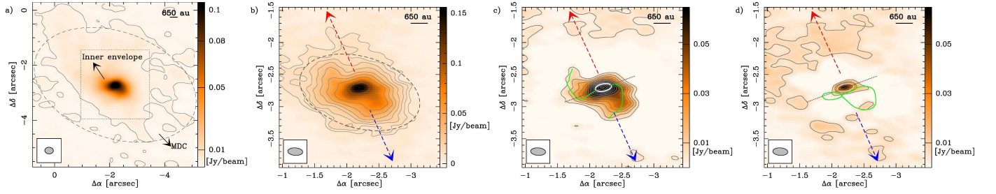
Fig. 2. A zoom on Fig. 1 of the protostar centred on \Delta\alpha = -2.17'' and \Delta\delta = -2.76'' offset from the phase center. a) Continuum emission smoothed to a resolution of 0.27'' showing the extended emission at the scale of the MDC. The color scale is linear between -1 and 105\text{ mJy/beam} , and the contour displays the 1.4\text{ mJy/beam} level corresponding to \sim 5\sigma . Dashed ellipse shows the FWHM of the MDC from Table 1 adopted from Csengeri et al. (2017b). The region of the inner envelope shown in panels b to c is outlined by a dashed box. The FWHM beam is shown in the lower left corner of all panels. b) Line-free continuum emission in the original, unsmoothed 12m and 7m array combined map where the beam has a geometric mean of 0.17'' . The color scale is linear between -3\sigma and 120\sigma , contours start at 7\sigma and increase on a logarithmic scale up to 120\sigma by a factor of 1.37 . The red and blue dashed lines show the direction of the CO outflow (see Fig. 7 and Sect. 3.4). The dark gray dashed ellipse shows 2\times the major and minor axes of the fitted 2D Gaussian. c) Residual continuum emission after removing a 2D Gaussian with a fixed lower peak intensity from the envelope component in order to enhance the contrast of the inner envelope. The color scale is linear from 0 to 50\sigma . The contours start at 3\sigma and increase by 6\sigma . White ellipse shows the FWHM of the fitted 2D Gaussian to the residual from panel b , and the green line outlines the azimuthal elongations. The black dotted line marks the direction perpendicular to the outflow. d) Residual continuum emission after removing the Gaussian fit to the envelope component (see the text for details). The color scale is the same as in panel c . Contours start at 5\sigma and increase by 10\sigma . Green contours show 80\% of the peak of the velocity integrated emission of the 334.436\text{ GHz } v_t = 1\text{ CH}_3\text{OH} line shown in Fig. 4.
