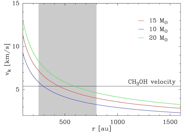
Fig. 14. Keplerian velocity as a function of radius, r , from the central object for 10, 15, and 20\ M_\odot . The projection corrected velocity determined from the 334.42 GHz \text{CH}_3\text{OH } v_t = 1 line is marked as a gray horizontal line. The grey shaded area corresponds to the projected distance range for the position of the \text{CH}_3\text{OH } v_t = 1 spots.
