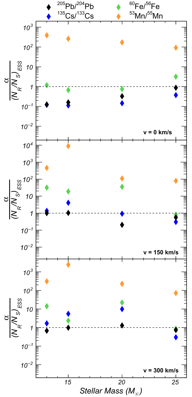
Figure 6. Predictions for SLRs from a late contamination by a CCSN in the mass range 13\text{--}25 M_{\odot} , assuming as a reference a solar ^{60}\text{Fe}/^{56}\text{Fe} ratio of 1 \cdot 10^{-6} . As the figure shows, in this second case the models with no rotation up to 20 M_{\odot} and the model of 25 M_{\odot} with a rather high rotation rate ( \geq 150 \text{ km s}^{-1} ) would account reasonably for ^{60}\text{Fe} (in addition to ^{26}\text{Al} and ^{41}\text{Ca} , which are used for fixing the parameters), avoiding overproductions for ^{107}\text{Pd} and ^{135}\text{Cs} . However, ^{53}\text{Mn} would remain, also in this case overproduced by two orders of magnitude, and would require a much larger mass cut, as in Meyer & Clayton (2000).
