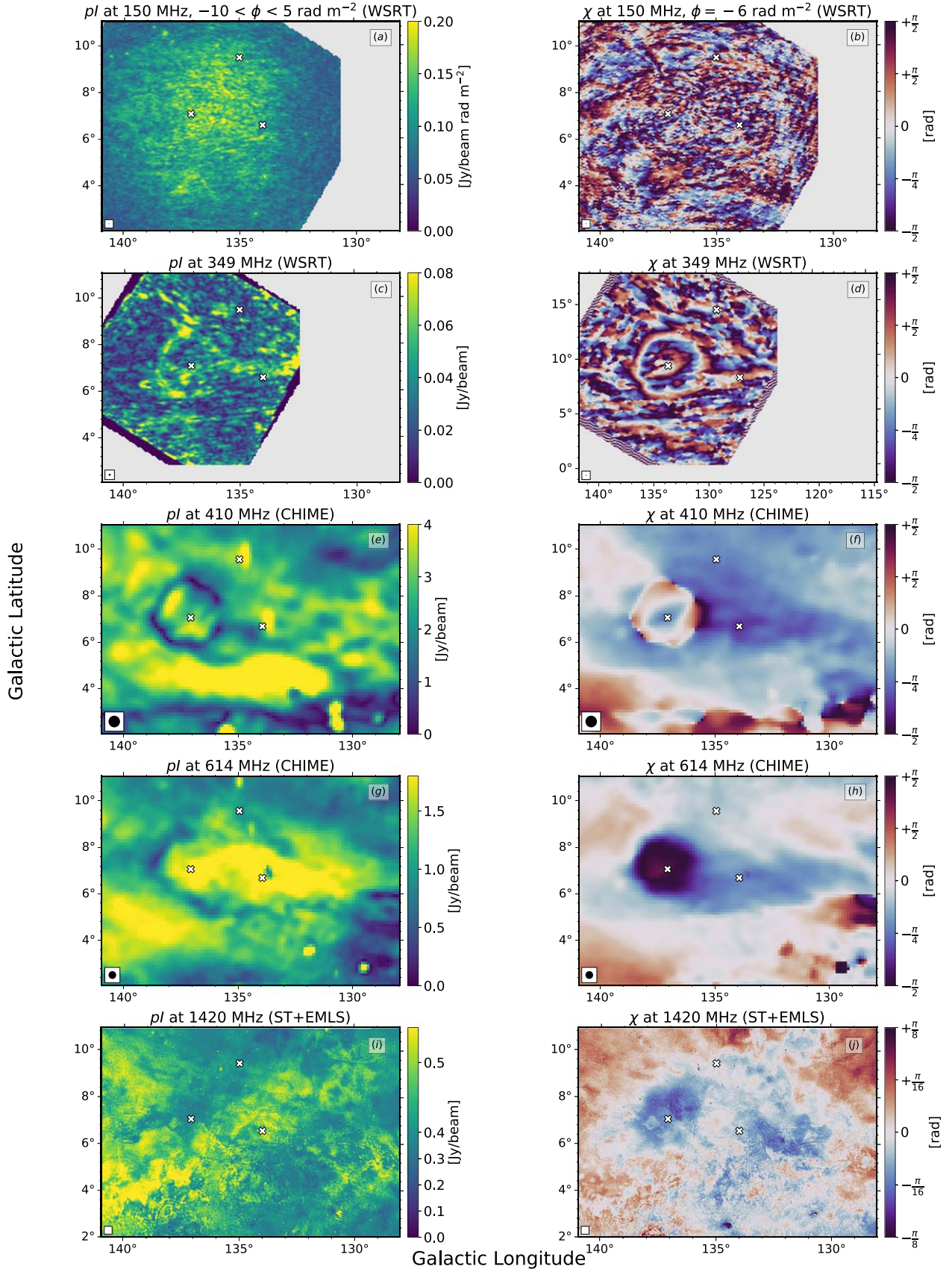
Figure 5. The tadpole depicted in polarized intensity (left) and polarization angle (right). From top to bottom: (a), (b) Bernardi et al. (2009) Faraday synthesis data at frequencies \sim 150\text{ MHz} with the WSRT at \phi = -2\text{ rad m}^{-2} (a frequency data cube is unavailable), (c), (d) Haverkorn et al. (2003) single-frequency polarized intensity and polarization angle at 349\text{ MHz} , CHIME data at (e), (f) 410\text{ MHz} and (g), (h) 614\text{ MHz} , and (i), (j) 1.4\text{ GHz} DRAO ST+EMLS data. "x" markers are as in Figure 2. Beams are shown within each image. Beams for the WSRT and ST+EMLS data are too small to be easily visible (see Table 1).
