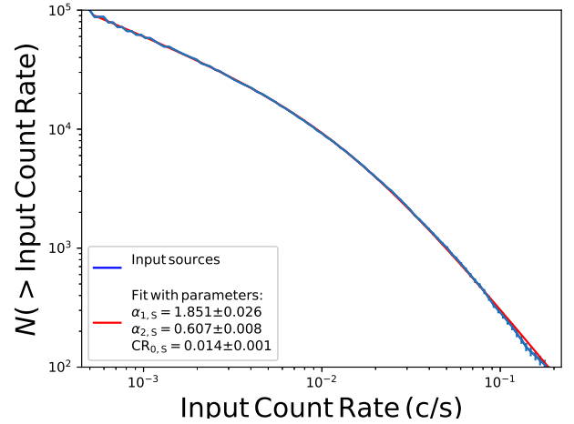
Fig. 13: \log(N(>CR)) - \log(CR) of input simulated point sources.
