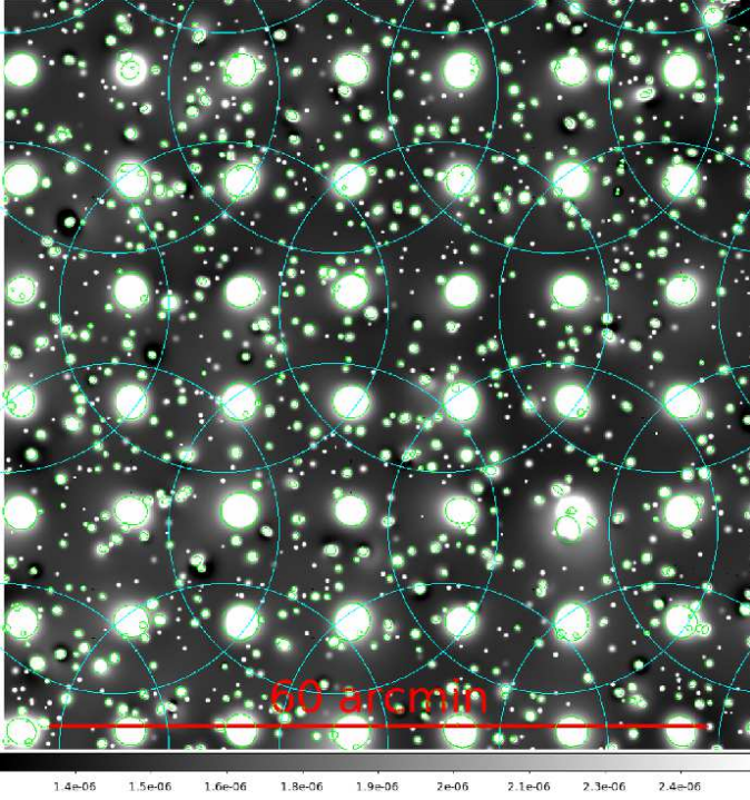
Fig. 3: 68' \times 68' combined (MOS1+MOS2+pn) tile smoothed with MR/1 on which preliminary source detection with SEXtractor has been run. The figure is the smoothed version of the left panel of Figure 2. Green circles indicate sources tentatively identified by SEXtractor. Detected sources include clusters (larger sources regularly spaced by 10' ) with count rates of 0.1 count/s and core radius 20'' , and resolved AGNs inserted at random positions (smaller sources irregularly spaced). The exposure time is 10 ks and background is added. Cyan circles represent the XMM pointings and are 15' in radius; the pointing geometrical centres at which the circles are drawn are not the same as the centres of the optics (points of maximum telescope sensitivity).
