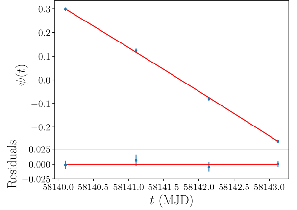
Figure 2. Phase drift \psi(t) of PSR J1023+0038 with respect to a uniform rotation with period P_{init} , fitted with a second-order polynomial (solid line). Time t is expressed in MJD. Residuals of the fit are shown in the bottom panel.
