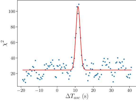
Figure 1. Epoch folding search of the time of passage at the ascending node for the 2018 January 25 Aqueye+ observation of PSR J1023+0038. Time is measured from the value of T_{asc} predicted using the orbital period from the X-ray ephemeris (Jaodand et al. 2016).
