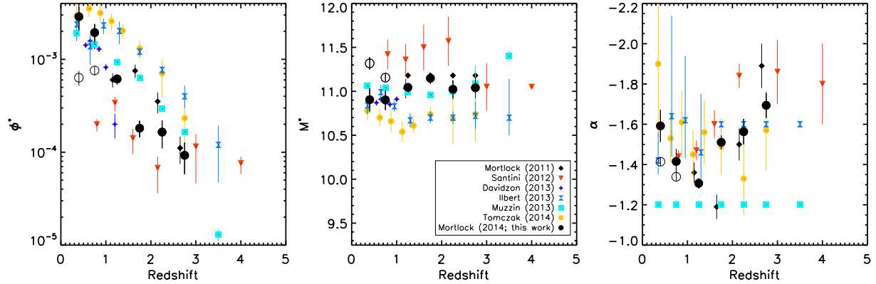
Figure 6. The Schechter function parameters of the fits shown in Fig. 5 (black filled circles). The black empty circles are from the single Schechter fits to the total galaxy SMF (not plotted in Fig. 5 but shown here for comparison). The black filled diamonds are the results from Mortlock et al. (2011), the blue filled squares are the results from Muzzin et al. (2013), the yellow filled circles are the results from Tomczak et al. (2014), the red filled triangles are the results from Santini et al. (2012), the blue filled bow ties are the results from Ilbert et al. (2013), and the blue filled stars are the results from Davidzon et al. (2013). Where necessary, we converted the literature values of M^* to a Chabrier IMF.
