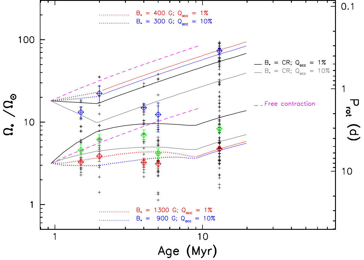
Fig. 5. Same as Fig. 4, but for \dot{M}_{\text{acc,init}} = 10^{-8} \text{ M}_\odot \cdot \text{yr}^{-1} . It is important to note that for the fast rotation cases, the black and red lines are superimposed.
