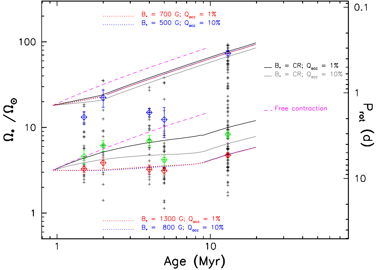
Fig. 4. Angular velocity evolution of stellar convective envelope as function of time for fast (up) and slow (down) rotator models in case where \dot{M}_{\text{acc,init}} = 10^{-9} \text{ M}_\odot \text{ yr}^{-1} . The black and the grey solid lines represent the MEs and APSW processes with Q_{\text{acc}} = 1\% and Q_{\text{acc}} = 10\% , respectively, and the magnetic field is from the BOREAS routine from Cranmer & Saar (2011). The red and the blue dotted lines represent the models including the MEs and APSW processes with Q_{\text{acc}} = 1\% and Q_{\text{acc}} = 10\% , respectively, but with the numerically imposed magnetic field B_{\text{mod}} . The free contraction (i.e. without any external interaction) is shown by the magenta long-dashed line. It represents the increase of the rotation rate during a free contraction phase. The angular velocity is scaled to the angular velocity of the present Sun. The blue and the red tilted square and associated error bars represent, respectively, the 90th percentile and the 25th percentile of the rotational distributions of solar-type stars in star-forming regions and young open clusters obtained with a rejection sampling method described in Gallet & Bouvier (2013).
