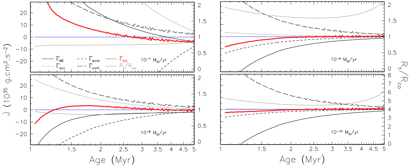
Fig. 6. Evolution of accretion torque \Gamma_{acc} (dotted line), ME’s torque \Gamma_{ME} (solid line), stellar wind torque \Gamma_{wind} (short dashed line), and positive torque due to stellar contraction (long dashed line) as function of time for median rotator with Q_{acc} = 1\% and \dot{M}_{acc,init} = 10^{-7} M_\odot.\text{yr}^{-1} (upper panel), \dot{M}_{acc,init} = 10^{-8} M_\odot.\text{yr}^{-1} (upper middle panel), \dot{M}_{acc,init} = 10^{-9} M_\odot.\text{yr}^{-1} (lower middle panel), and \dot{M}_{acc,init} = 10^{-10} M_\odot.\text{yr}^{-1} (lower panel). The red solid line is the sum of all of these torque contributions. The blue solid line represents the zero torque condition leading to a constant angular velocity during the disk accretion phase. The grey solid line shows the evolution of R_t/R_{co} .
