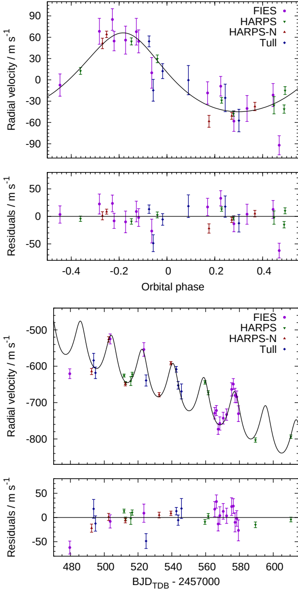
Figure 3. Radial velocities as a function of orbital phase ( upper panels ) and time ( lower panels ), with best-fitting models, and residuals to those models plotted below. Data points (with 1\sigma error bars) are from four different spectrographs, represented by different colours and symbol types.
