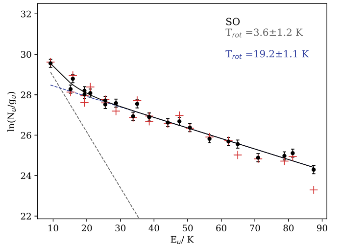
Figure 3. Similar to Figure 1 for SO. The best-fit LTE components are remarkably similar to those found for ^{34}\text{SO} . The overplotted red points indicate the upper state column density derived from the RADEX best-fit fluxes to give an indication of the quality of the RADEX fit.
