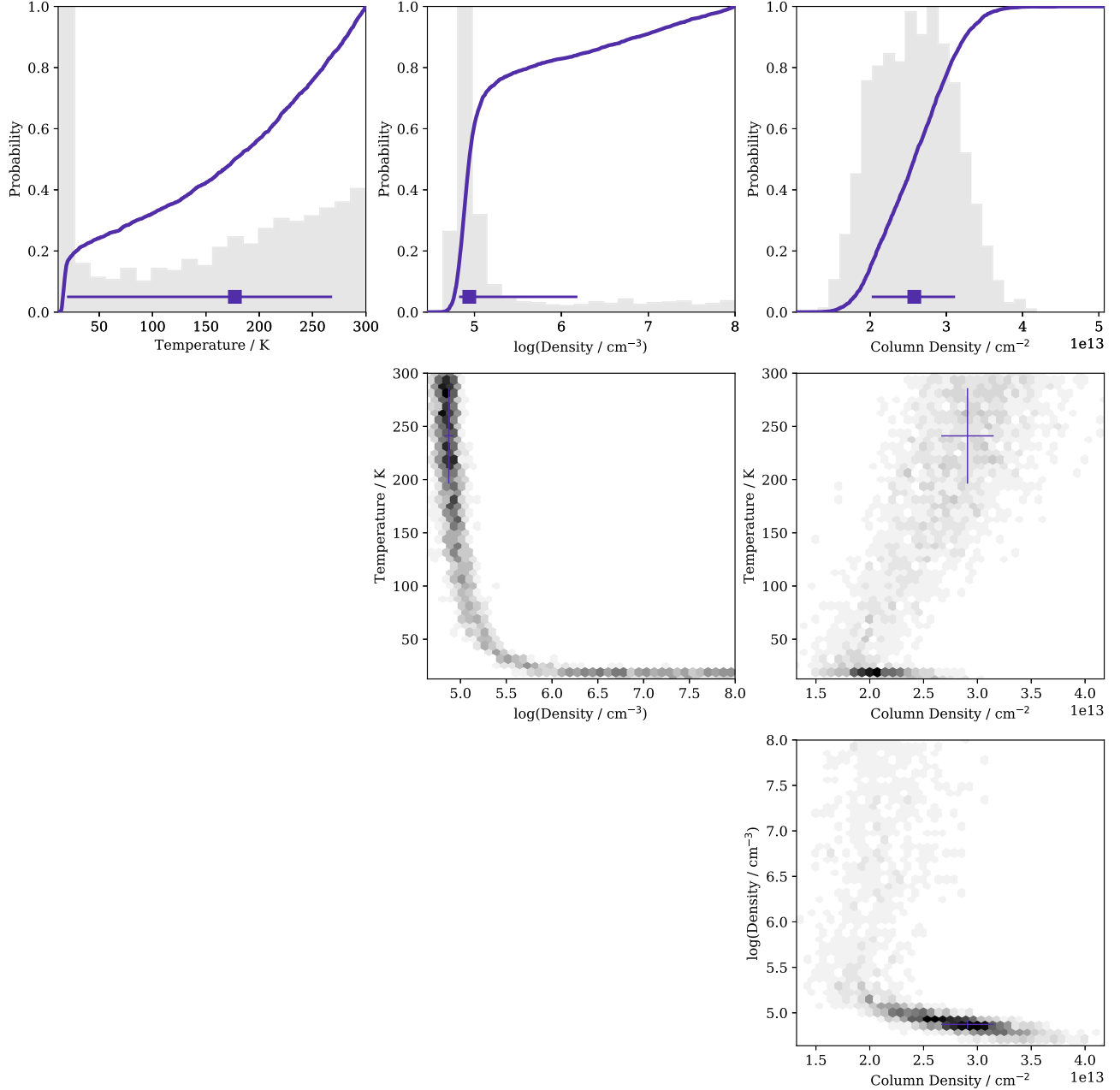
Figure 23. Probability distributions for \text{o-H}_2\text{CS} . The horizontal spans in the top row and the crosses in the lower panels show the position of the median of the distribution and 67% probability intervals for each parameter. The gray histograms show the probability density and the line shows the cumulative probability distribution. The gray scale in the lower panels shows the joint probability distribution of each parameter pair with darker areas representing higher likelihoods. The column densities demonstrate the general trend of having a most likely value that is not strongly dependent on density and temperature.
