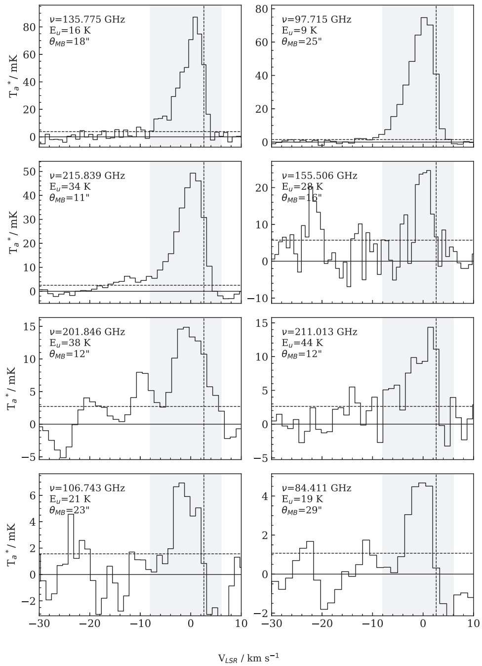
Figure 17. Similar to Figure 8 for detected ^{34}\text{SO} lines.
