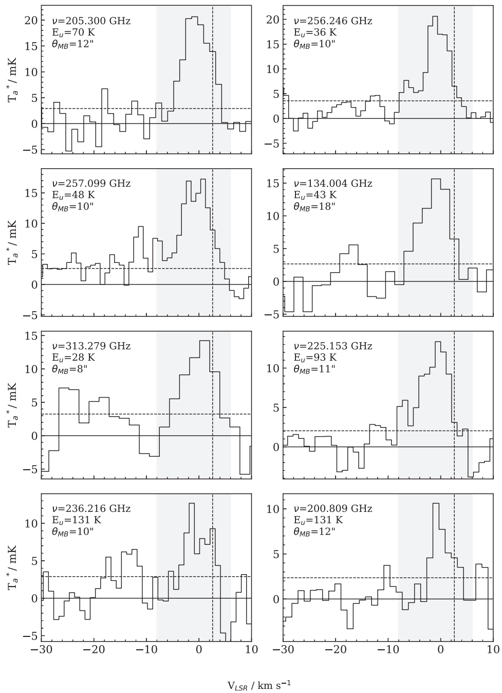
Figure 21. Detected \text{SO}_2 lines continued.
