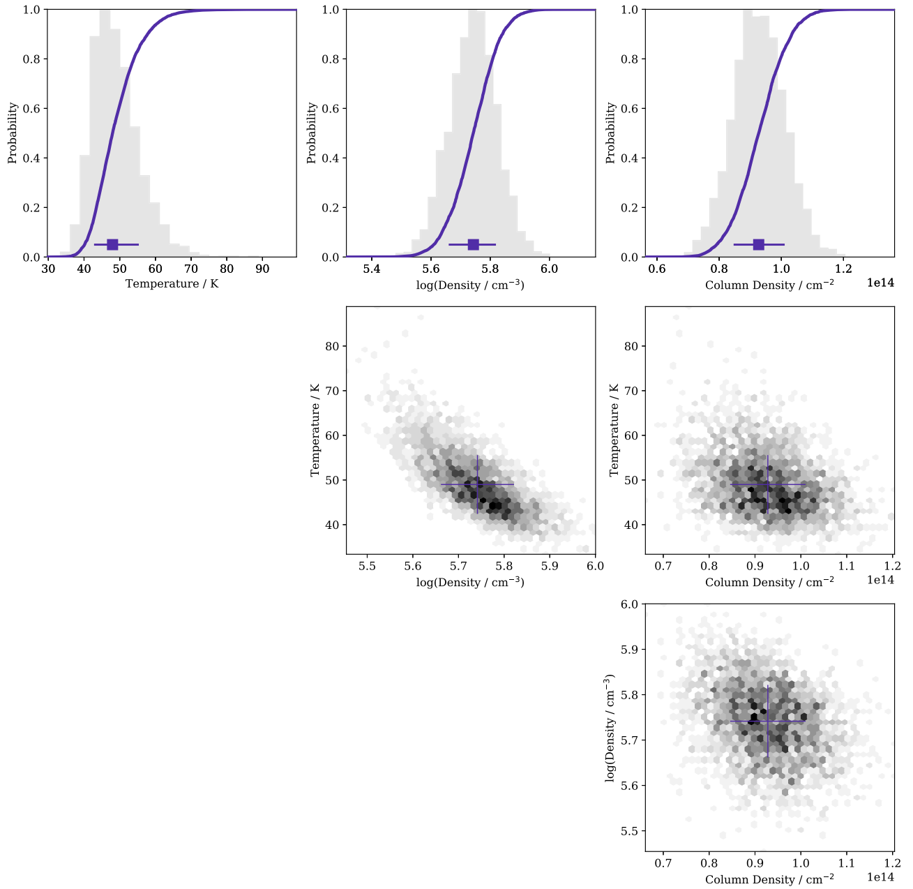
Figure 28. Same as Figure 23 but for SO 2 . SO 2 is unique in that it shows a single peaked distribution for all input parameters.
