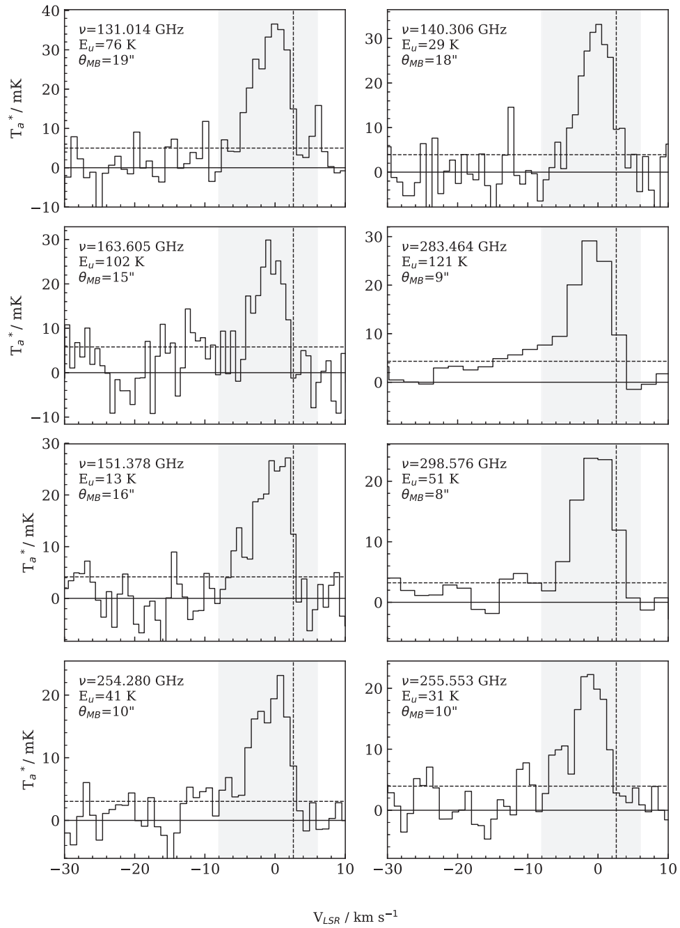
Figure 20. Detected \text{SO}_2 lines continued.
