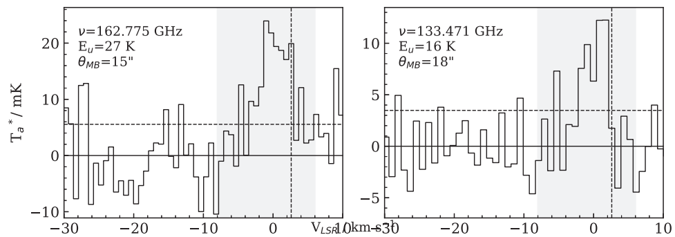
Figure 22. Similar to Figure 8 for detected ^{34}\text{SO}_2 lines.
