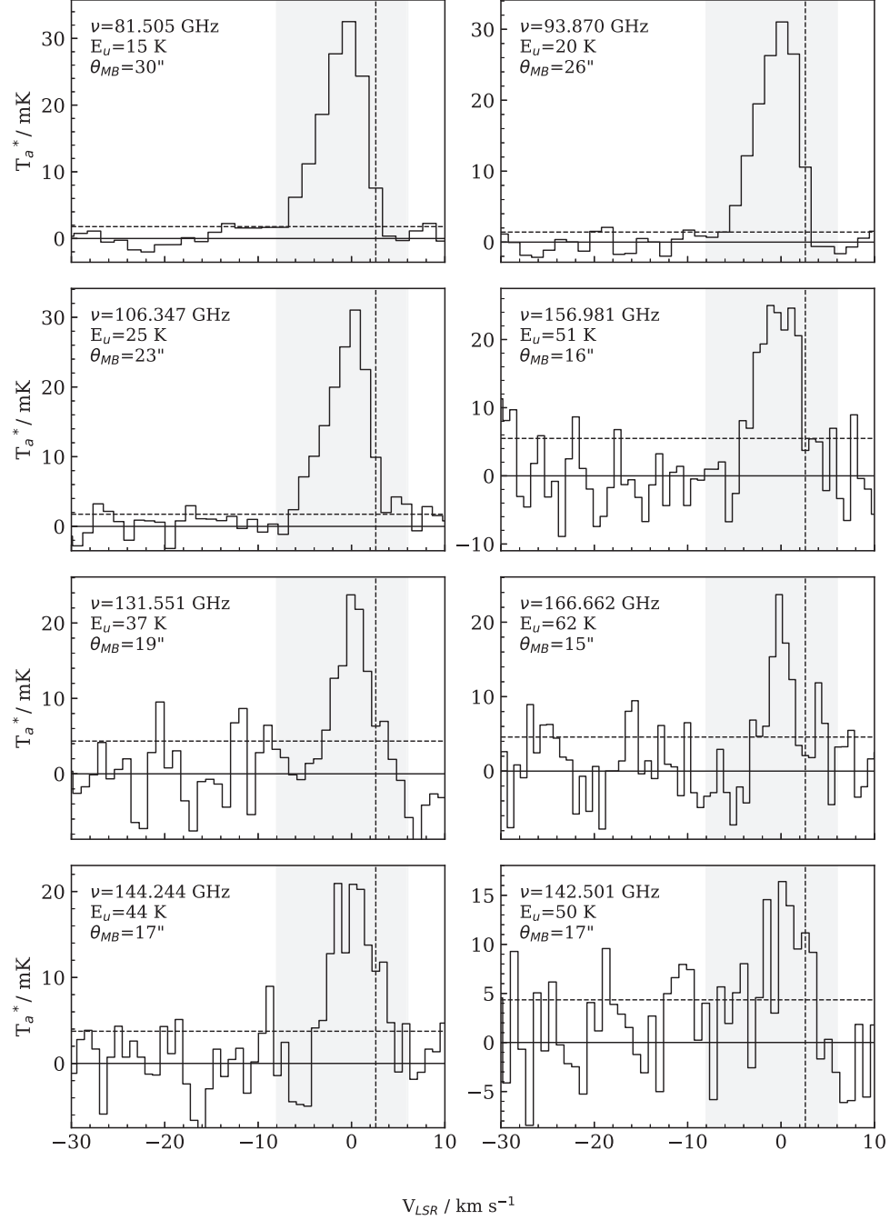
Figure 8. Detected CCS lines. Rows share Y-axis values, which are given in antenna temperature. The vertical black dashed line indicates the location of the local standard of rest velocity 2.6 km s -1 . The horizontal dashed line shows the 1 \sigma level for that spectrum. The shaded area shows the moderate velocity regime over which the spectra were integrated.
