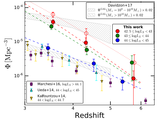
Figure 20. Comoving space density of three luminosity classes of AGN, divided in three redshift bins ( z = 3\text{--}4 , 4\text{--}5 , 5\text{--}6 ). The points are located at the weighted average redshift of each subsample. For the low-luminosity bin, the empty circles indicate the results derived applying the correction factors described in Section 4. At higher luminosities, the corrections have negligible effects, and are not shown for clarity. Since high-luminosity sources are not well sampled by the deep, pencil-beam fields used in this work, we report previous results in similar luminosity bins derived analysing data from wider fields. The dashed curves are the best-fitting models described in Section 6. The dotted curve is the best-fitting model for the low-luminosity bin, after the correction for incompleteness. The space density of galaxies in two different mass regimes from Davidzon et al. (2017), rescaled by an arbitrary factor of 0.02, is shown as a grey stripe.
