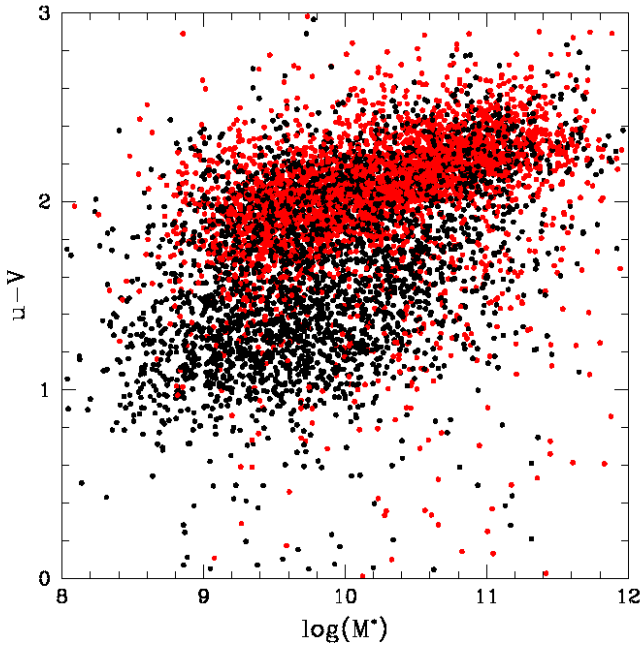
Fig. 12. u - V color versus stellar mass of the galaxies in log units. The red dots mark the galaxies with measured \text{SFR} = 0 , while the black dots those with \text{SFR} \neq 0 .
