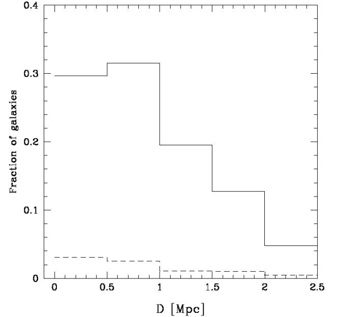
Fig. 13. Fraction of galaxies with \text{SFR} = 0 (solid line) at different cluster-centric distances. The measurement of the \text{SFR} = 0 is that provided by SINOPSIS (Fritz et al. 2007). The dashed line shows the same fraction but for the galaxies for which u - V < 1.5 .
